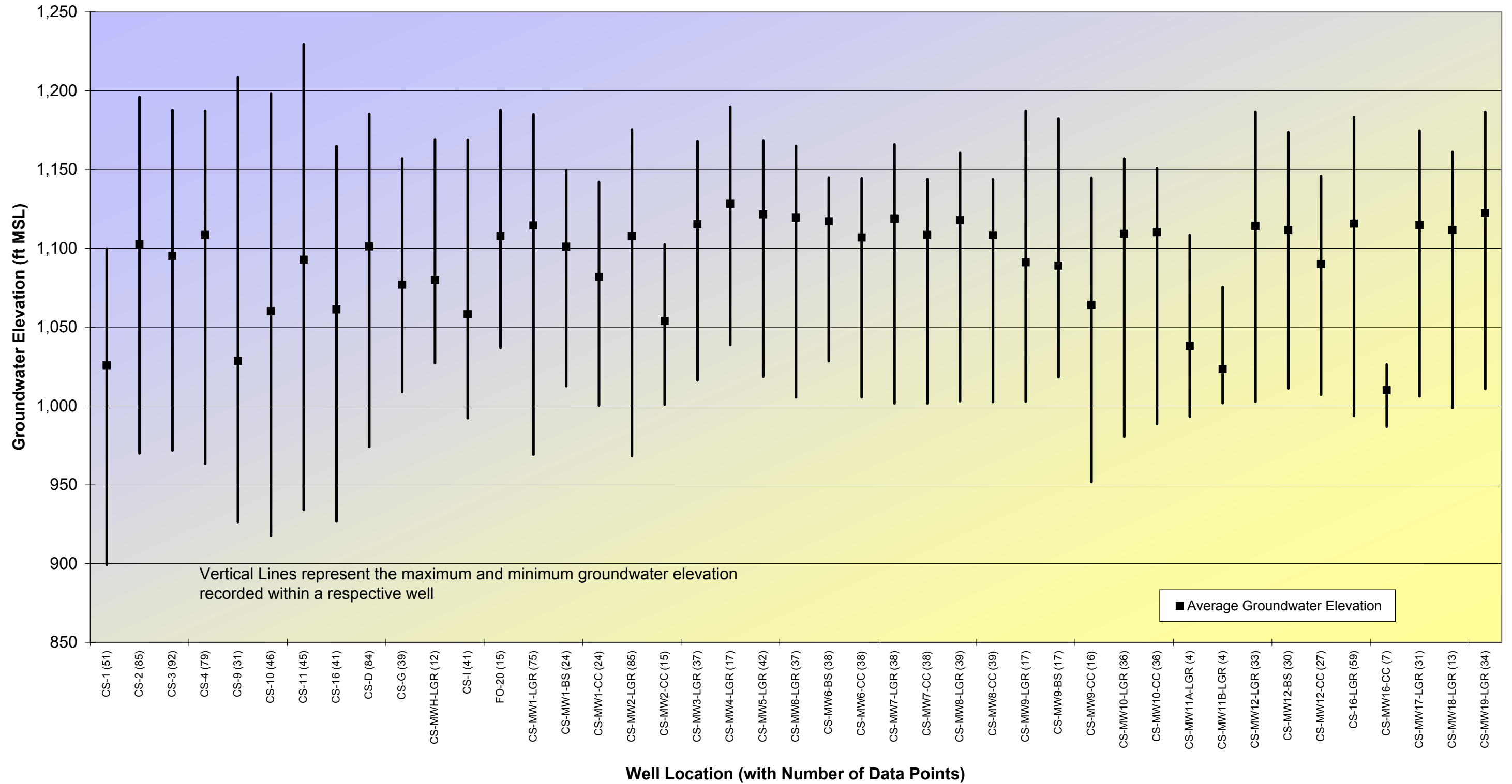
Figure 4.21 Range of Groundwater Elevations in Selected Wells 1992-2004 Camp Stanley Storage Activity - Boerne, TX
