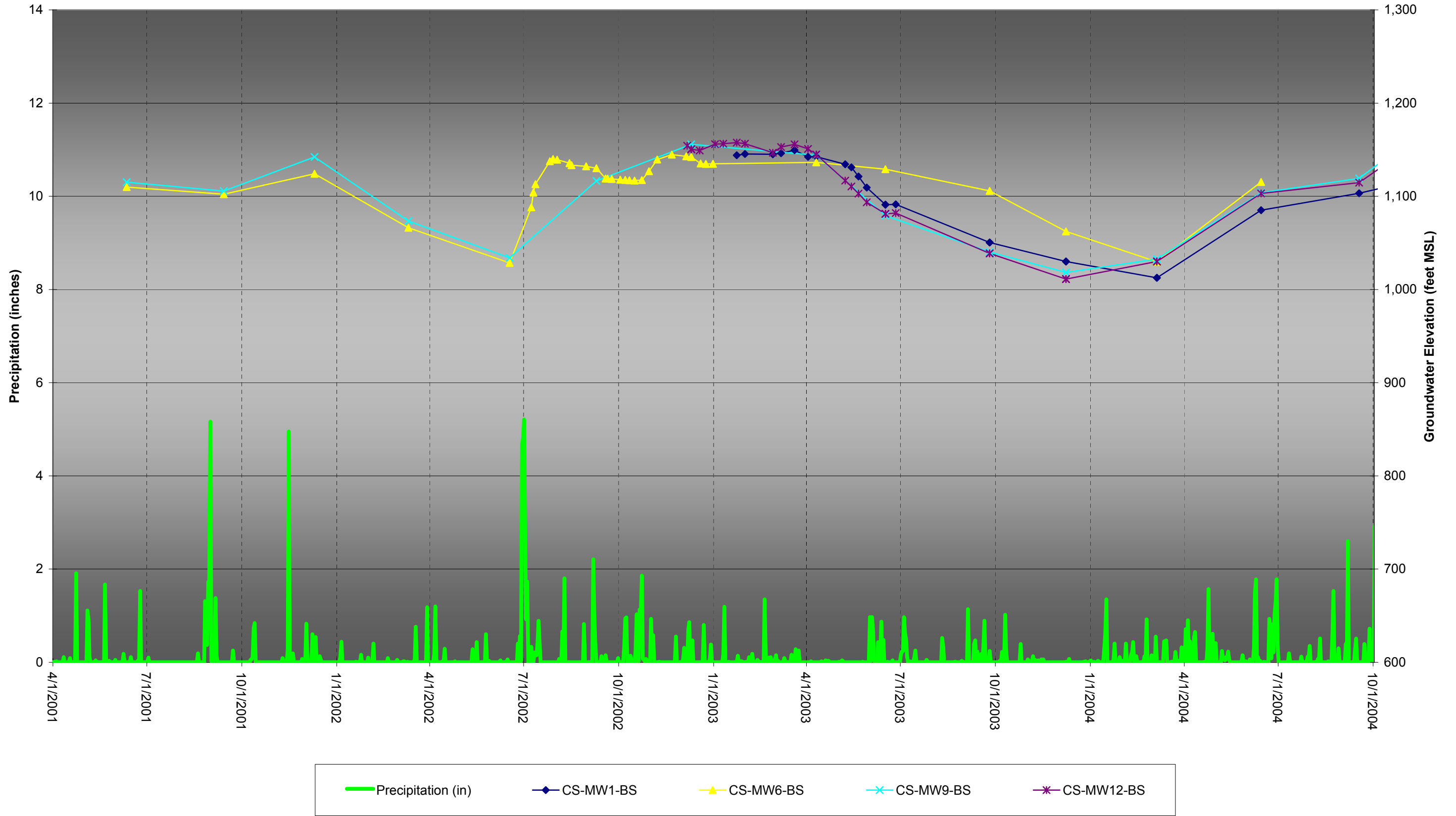
Figure 4.18 Hydrograph of Wells with Bexar Shale Completions December 1998 through September 2004
