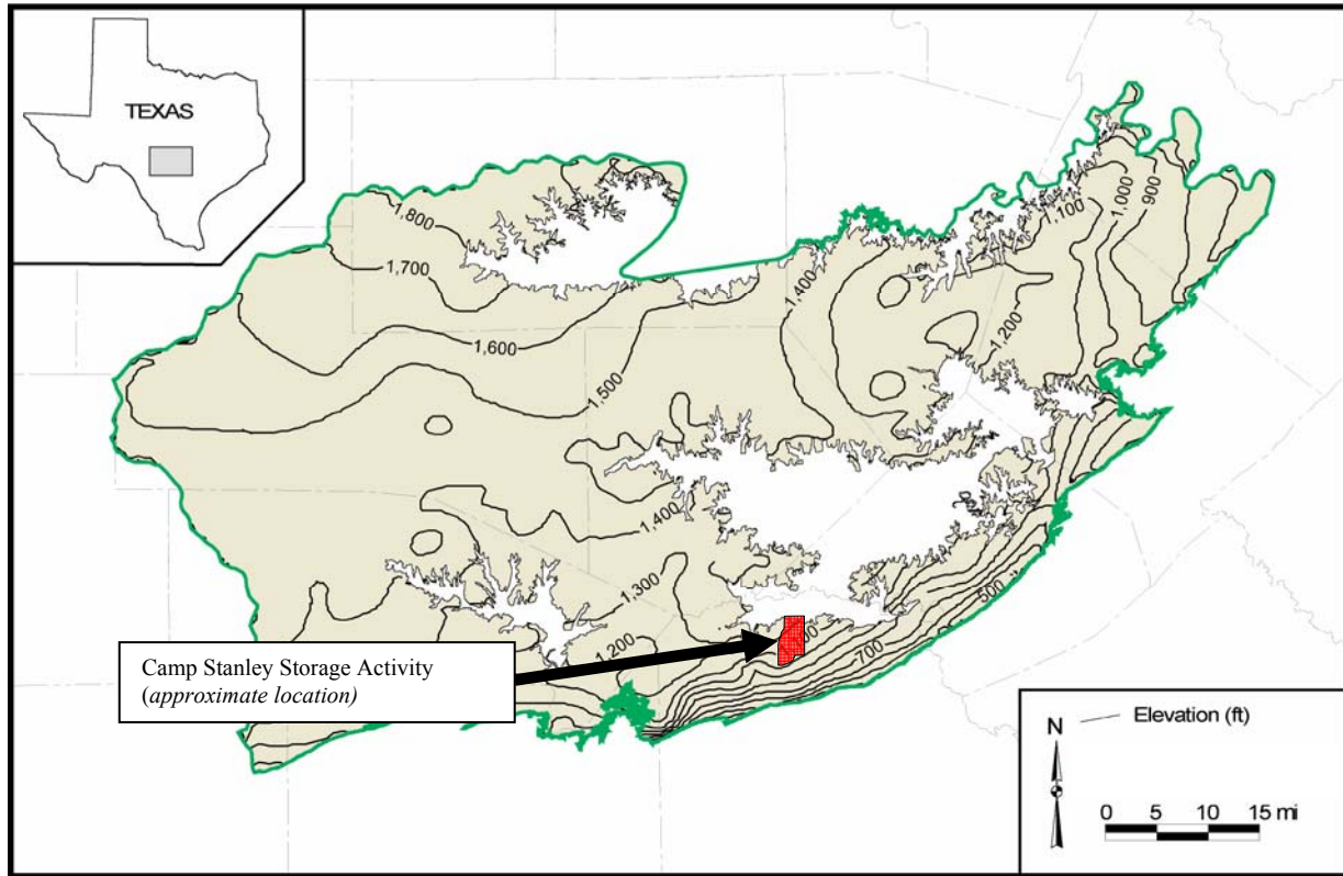
Figure 2.9 Elevation of the Base of the Upper Trinity Aquifer
