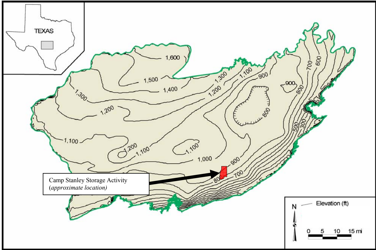
Figure 2.7 Elevation of the Base of the Middle Trinity aquifer
