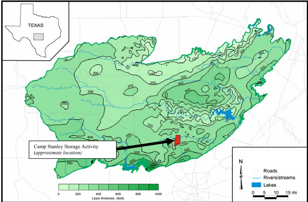
Figure 2.6 Approximate Thickness of the Middle Trinity aquifer
