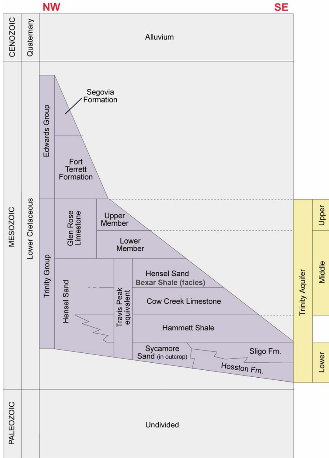
Figure 2.3 Stratigraphic and Hydrostratigraphic Section of the Hill Country Area
