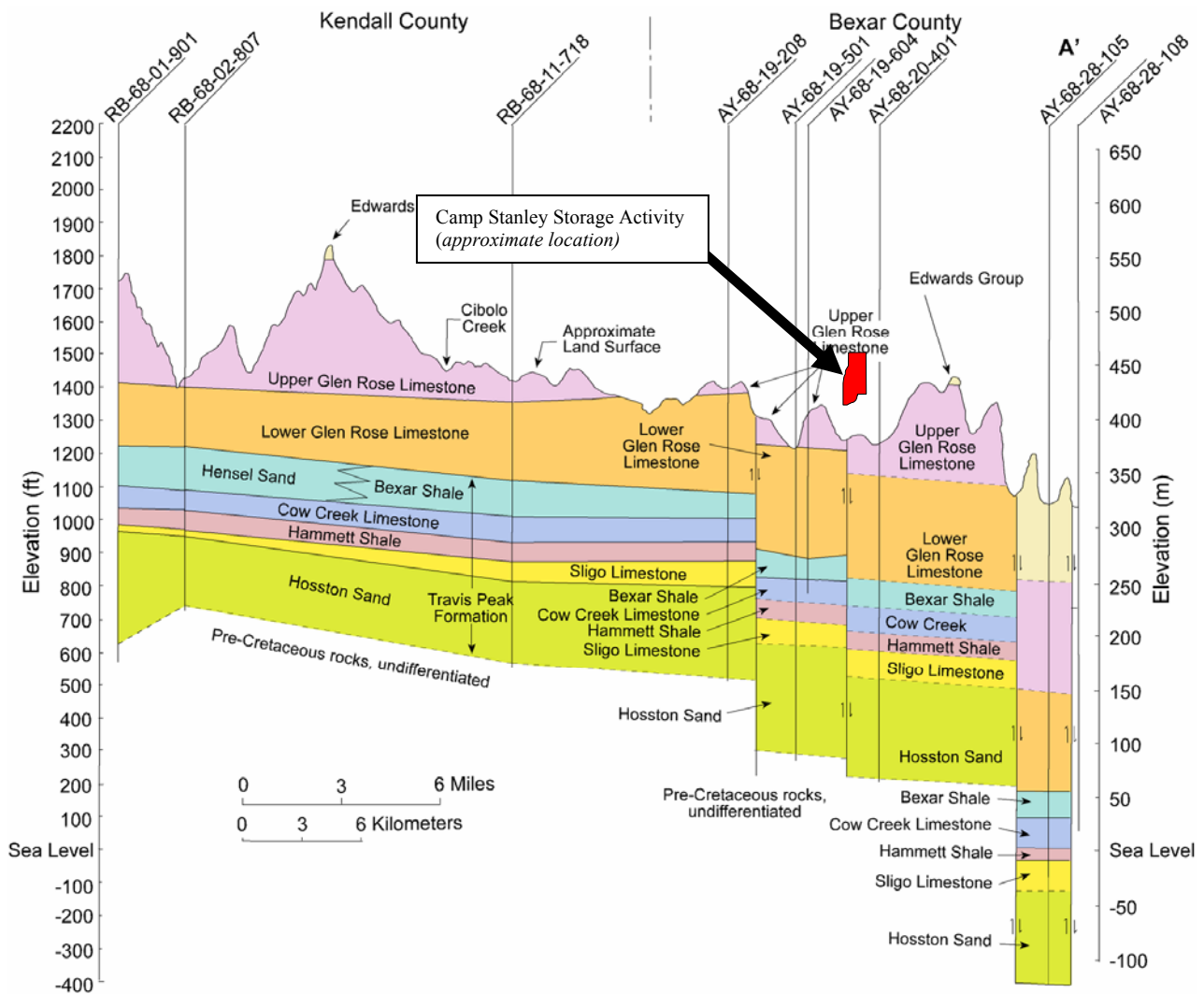
Figure 2.5 Geologic Cross Section through the Study Area
