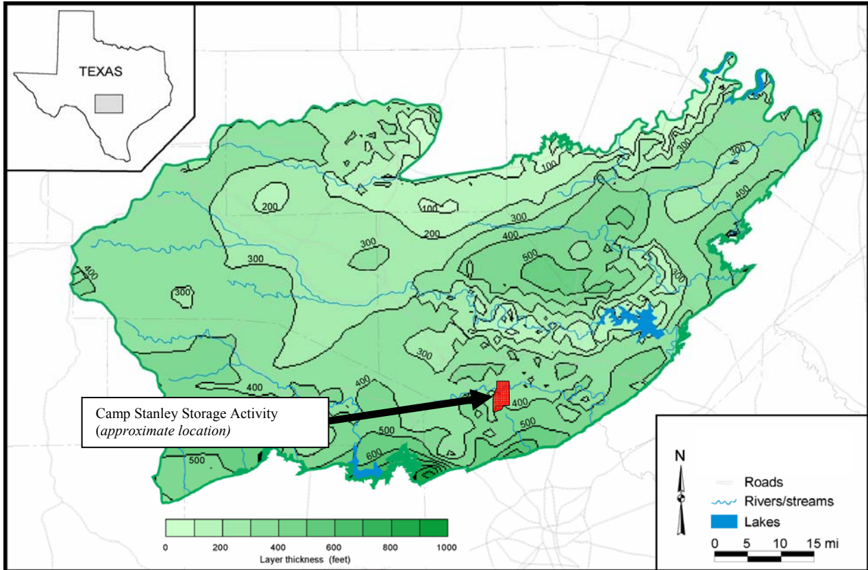
Figure 2.6 Approximate Thickness of the Middle Trinity aquifer
