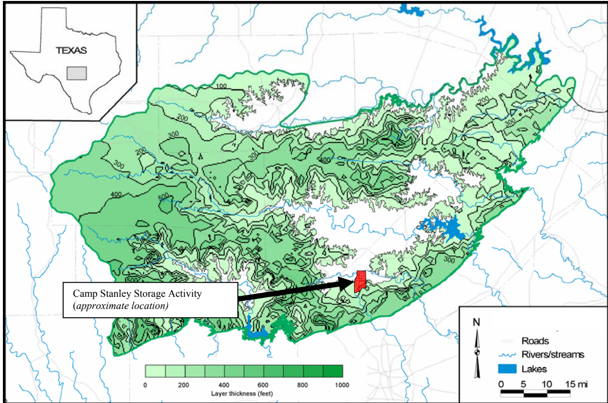
Figure 2.8 Approximate Thickness of the Upper Trinity aquifer
