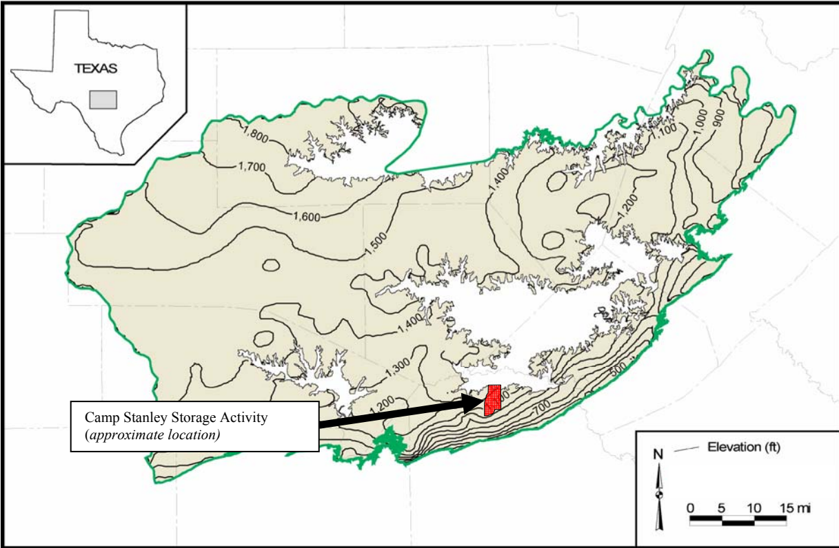
Figure 2.9 Elevation of the Base of the Upper Trinity Aquifer
