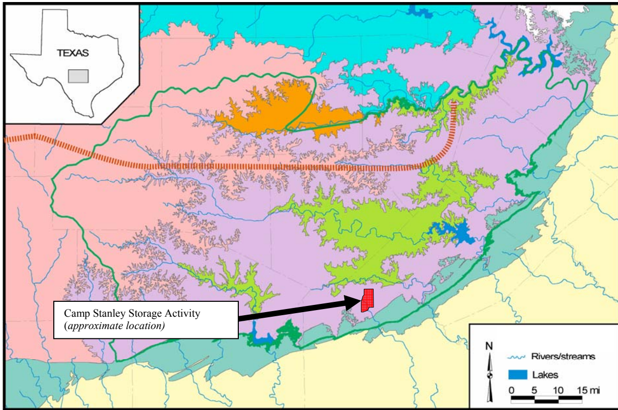
Figure 2.4 Surface Geologic Map
