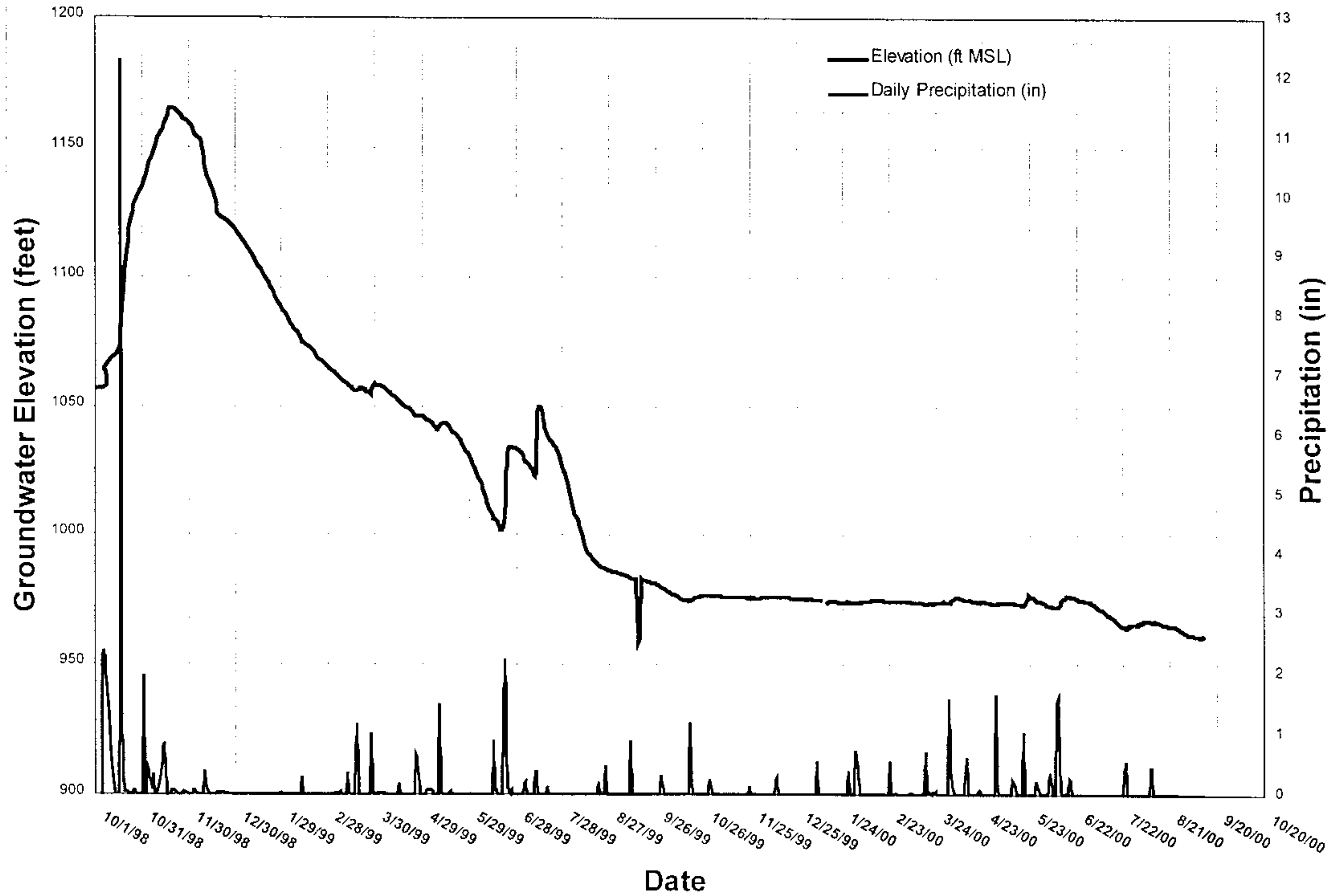
Figure 5 - Well 16 Groundwater Elevation and Precipitation Data Camp Stanley Storage Activity, Texas
