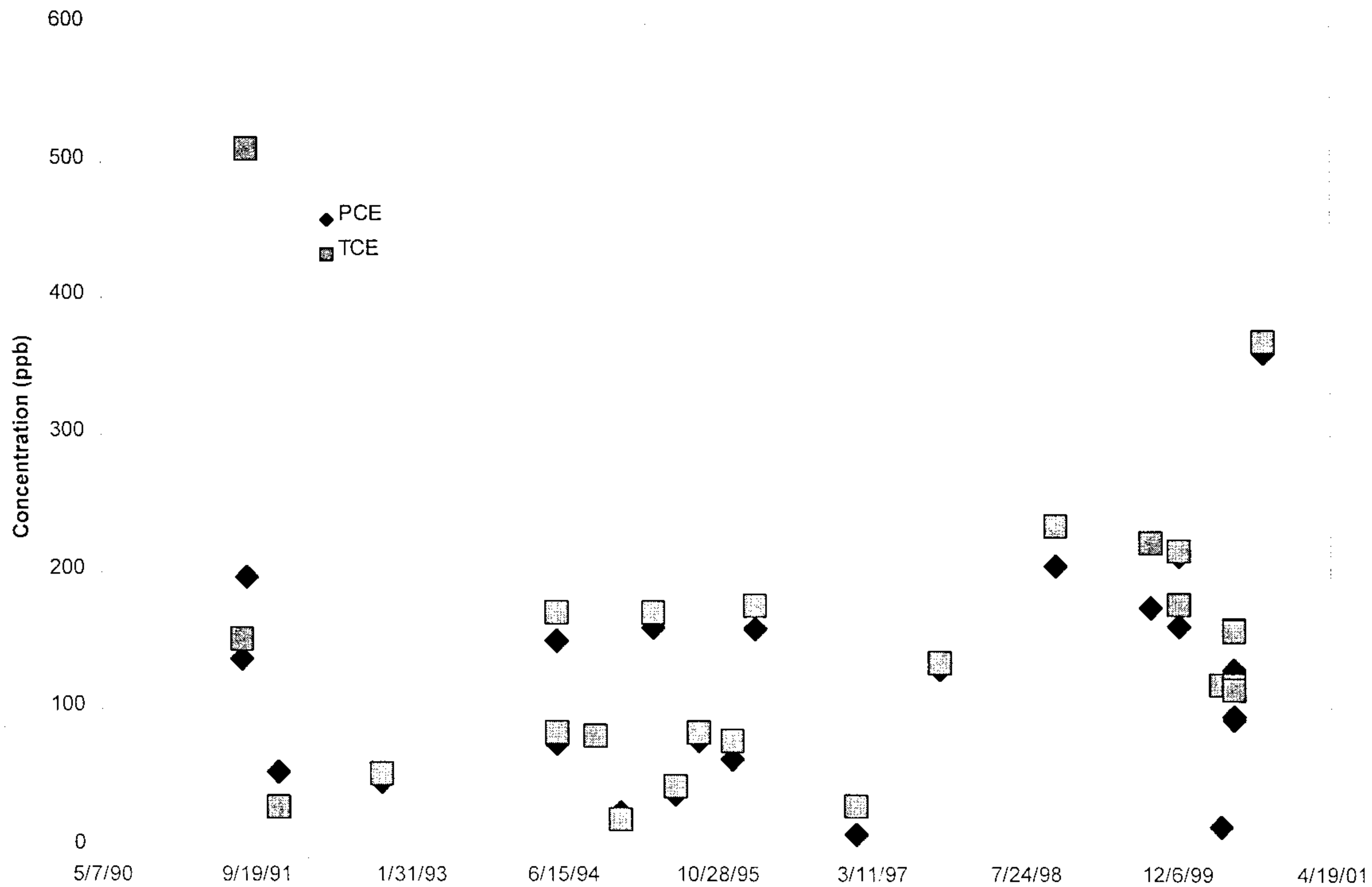
Figure 4 Well 16 Solvent Concentrations
