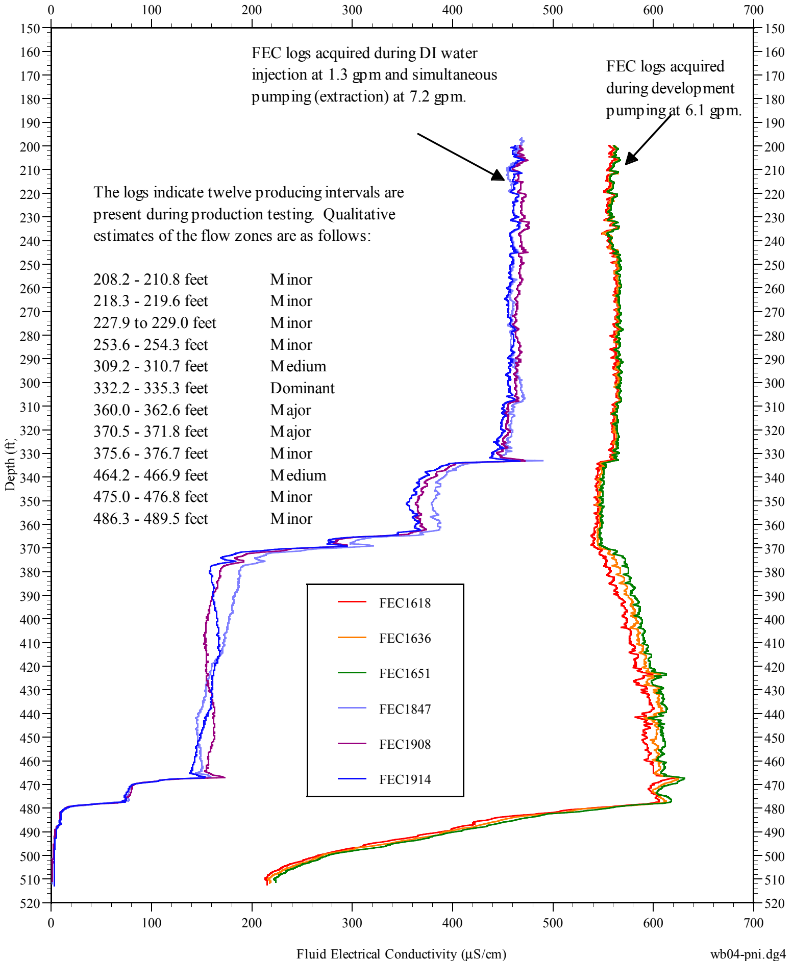
Figure 4.20 Summary of CS-WB04 Hydrophysical Logs During Low-Rate Production
