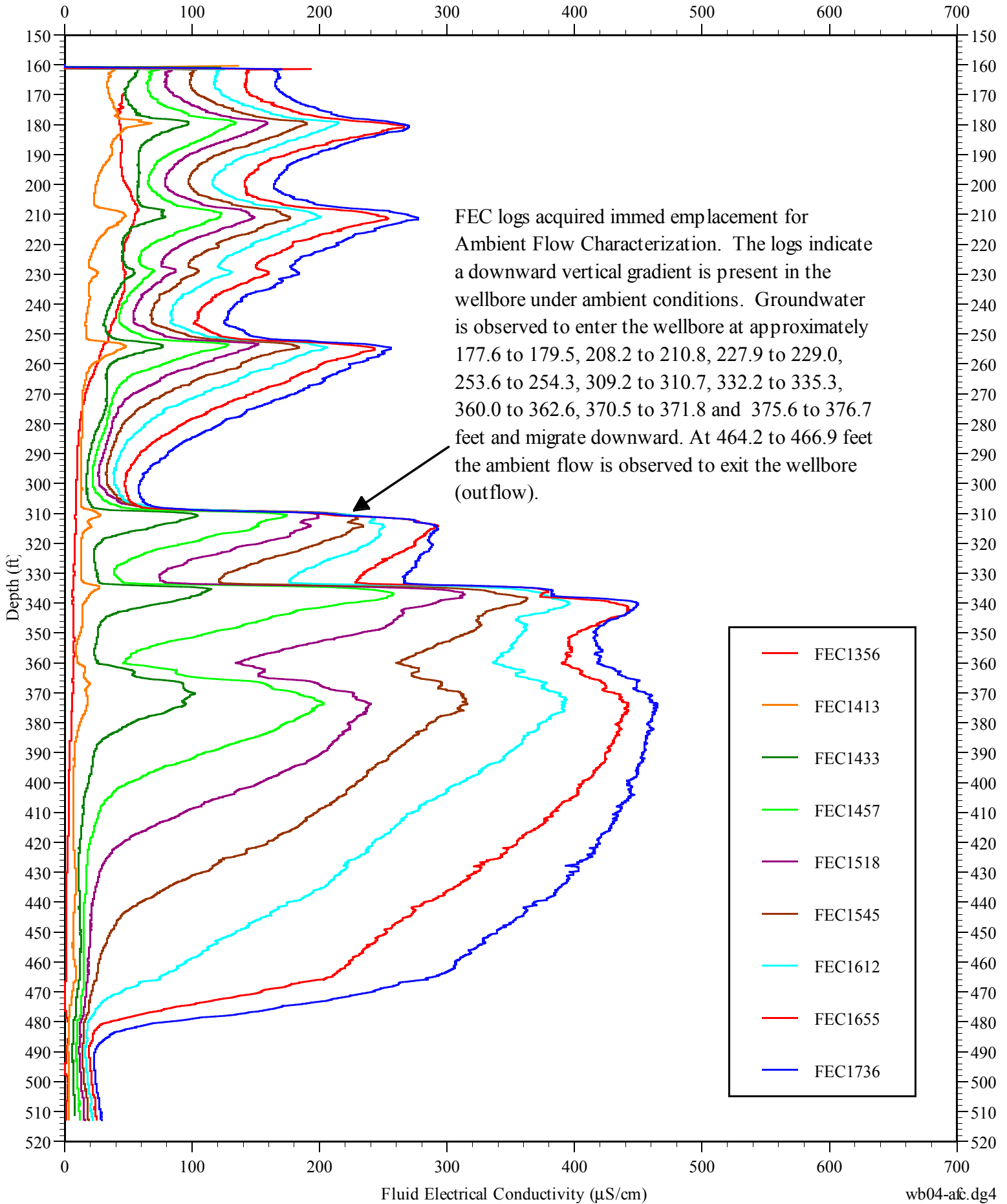
Figure 4.19 Summary of CS-WB04 Hydrophysical Logs During Ambient Flow Test
