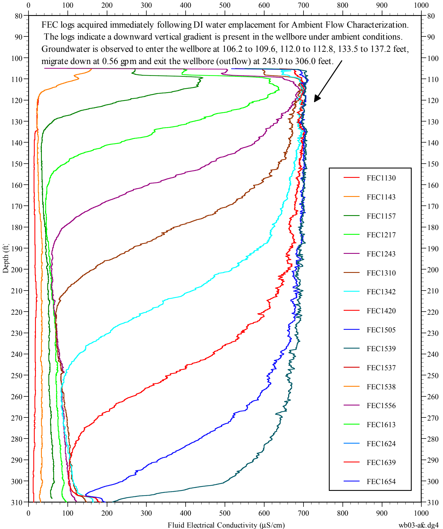
Figure 4.17 Summary of CS-WB03 Hydrophysical Logs During Ambient Flow Test
