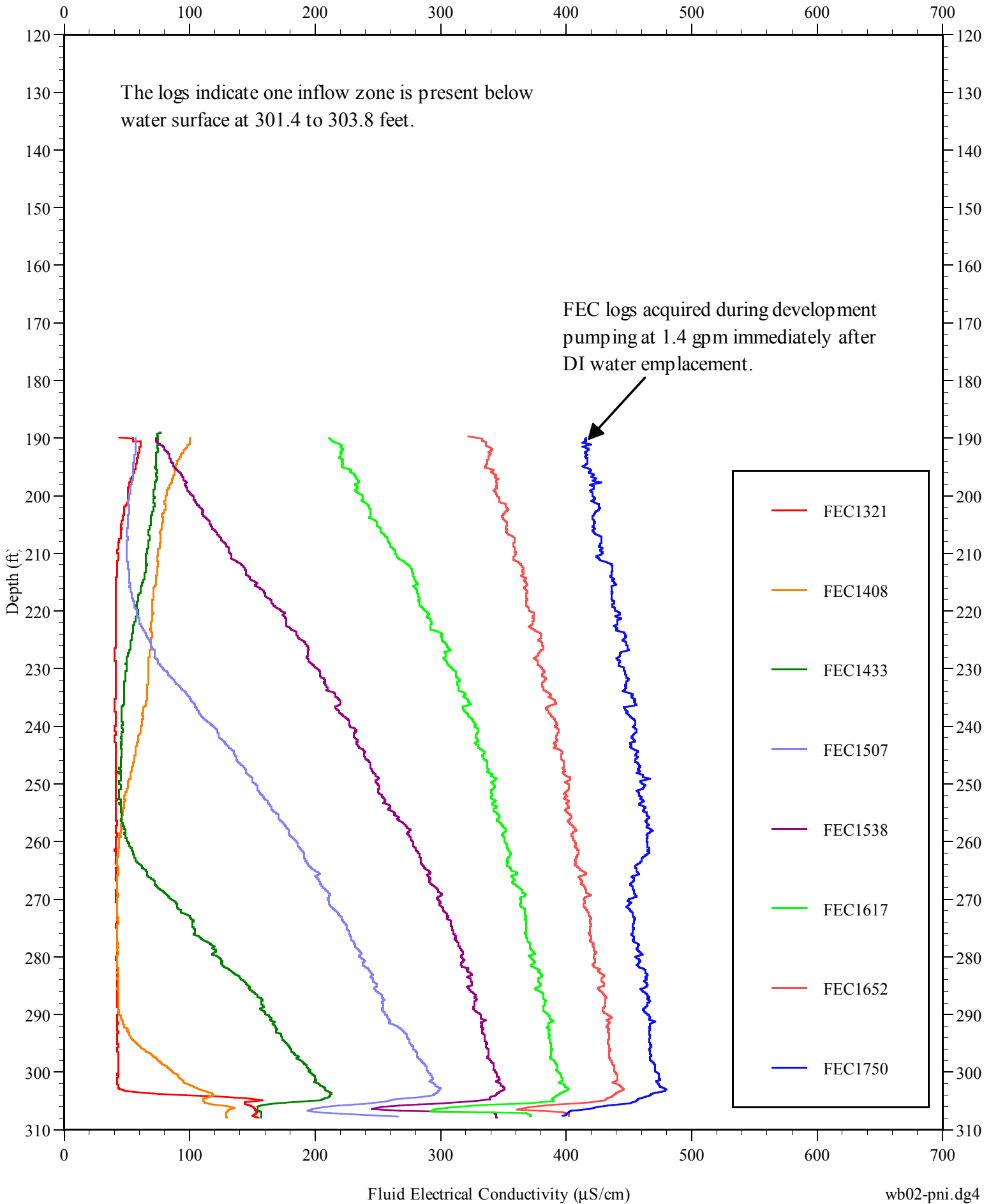
Figure 4.16 Summary of CS-WB02 Hydrophysical Logs During Low-Rate Production
