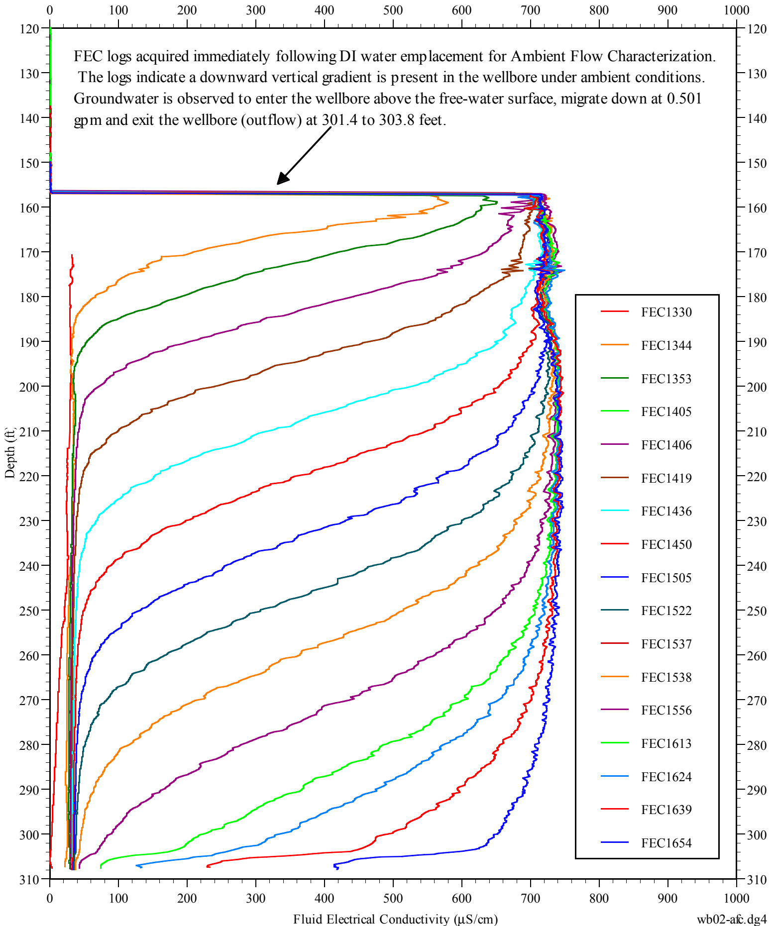
Figure 4.15 Summary of CS-WB02 Hydrophysical Logs During Ambient Flow Test
