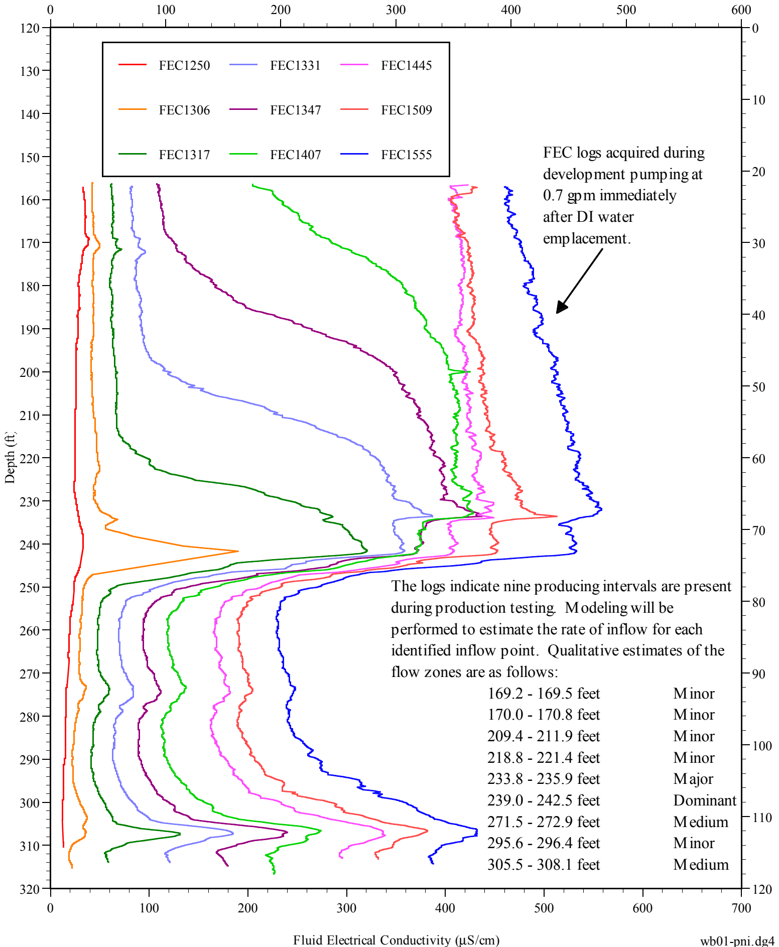
Figure 4.14 Summary of CS-WB01 Hydrophysical Logs During Low-Rate Production
