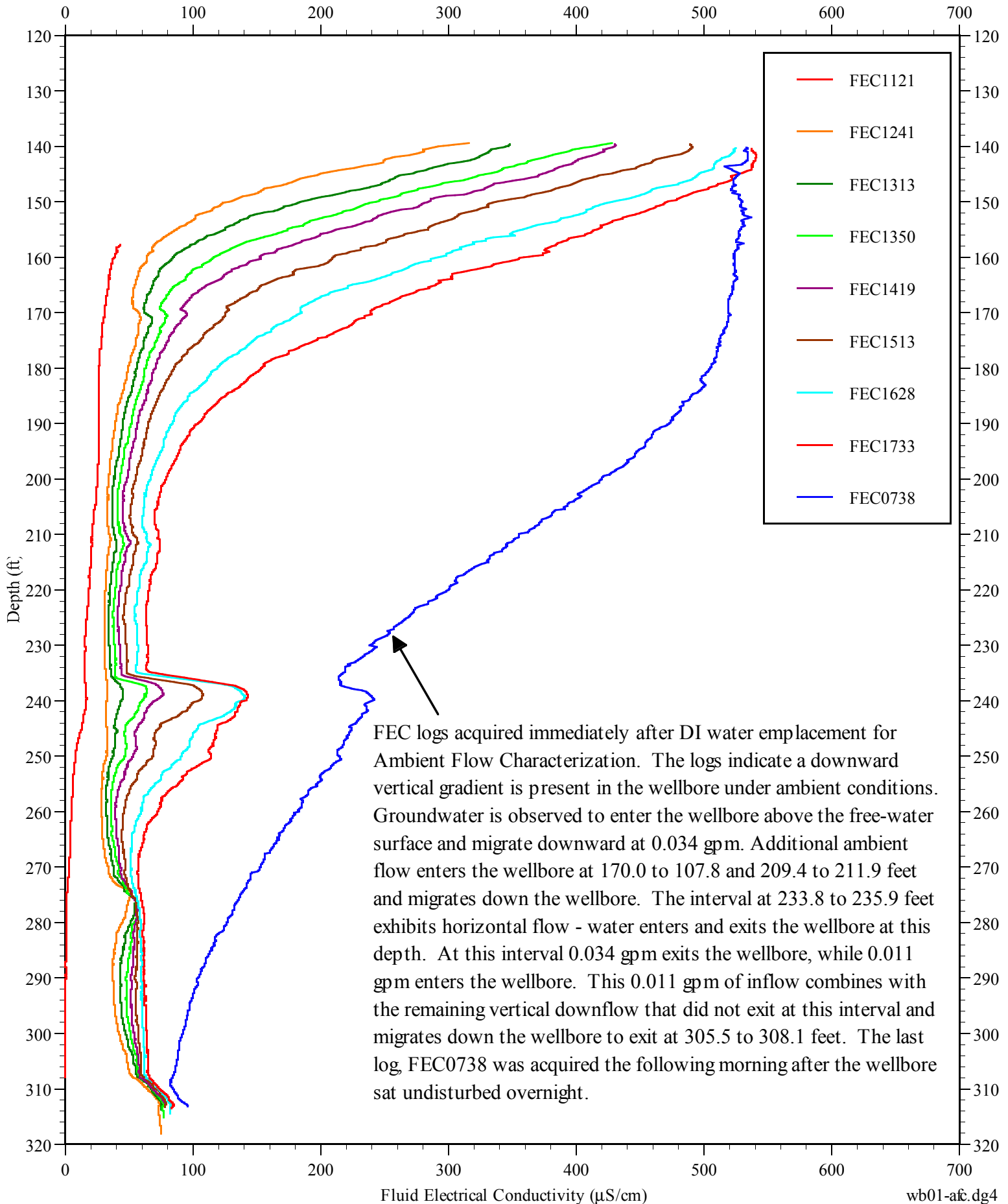
Figure 4.13 Summary of CS-WB01 Hydrophysical Logs During Ambient Flow Test
