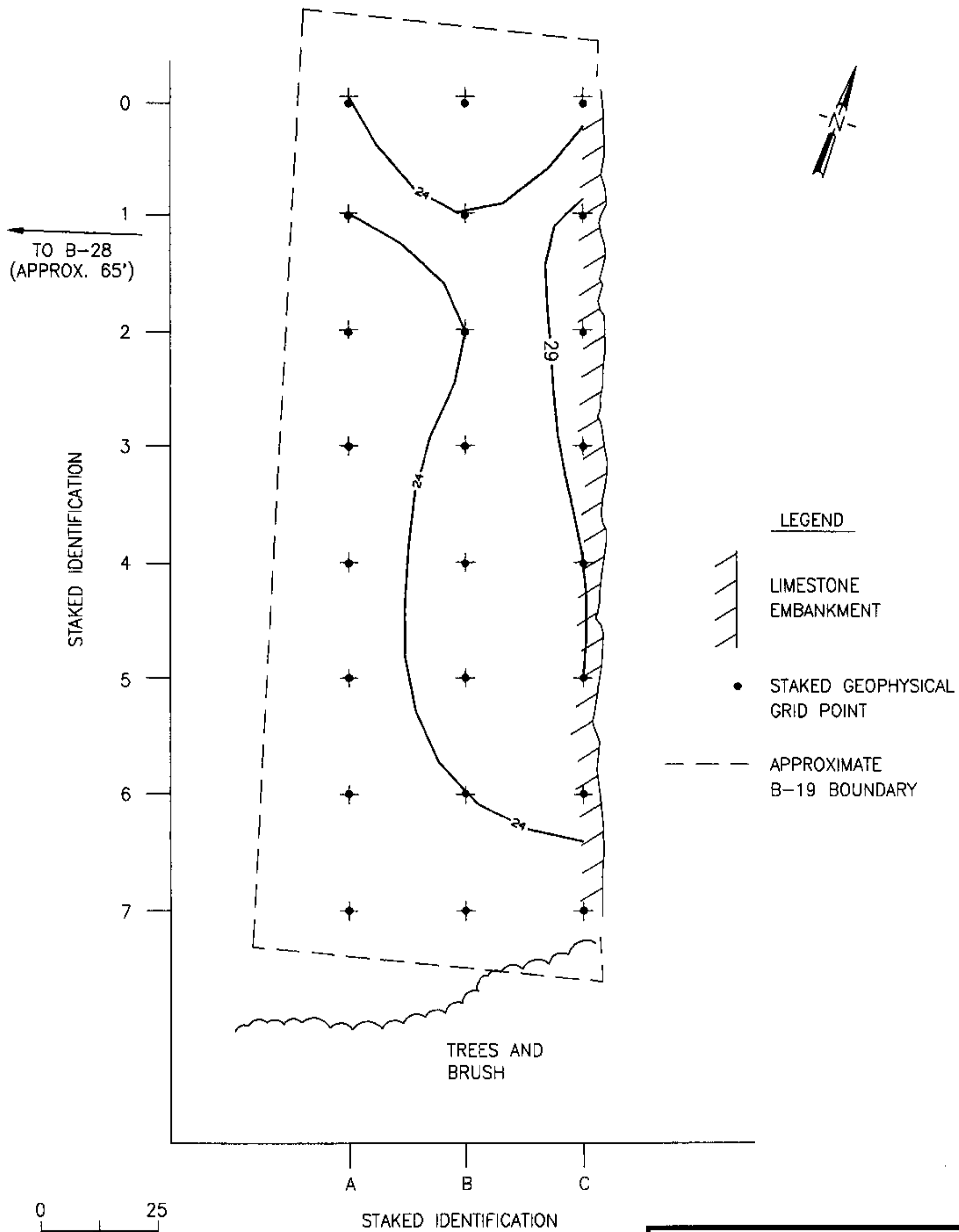
FIGURE 7.2 EM CONDUCTIVITY DATA SWMU B-19 CSSA GROUNDWATER EVALUATION
