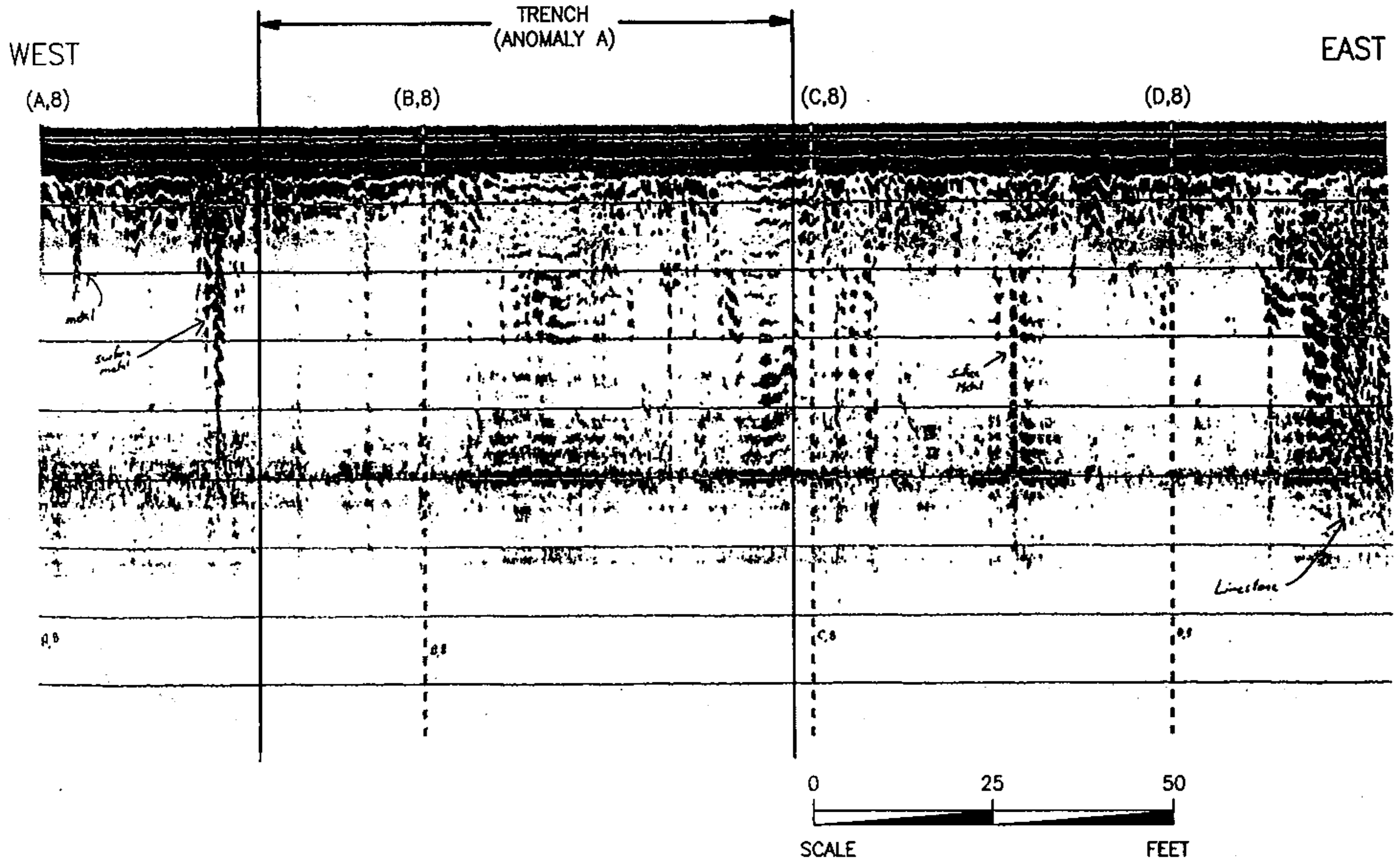
FIGURE 5.5 GSSI SIR-3 GPR PROFILE (LINE 8) SWMU B-4 CSSA GROUNDWATER EVALUATION
