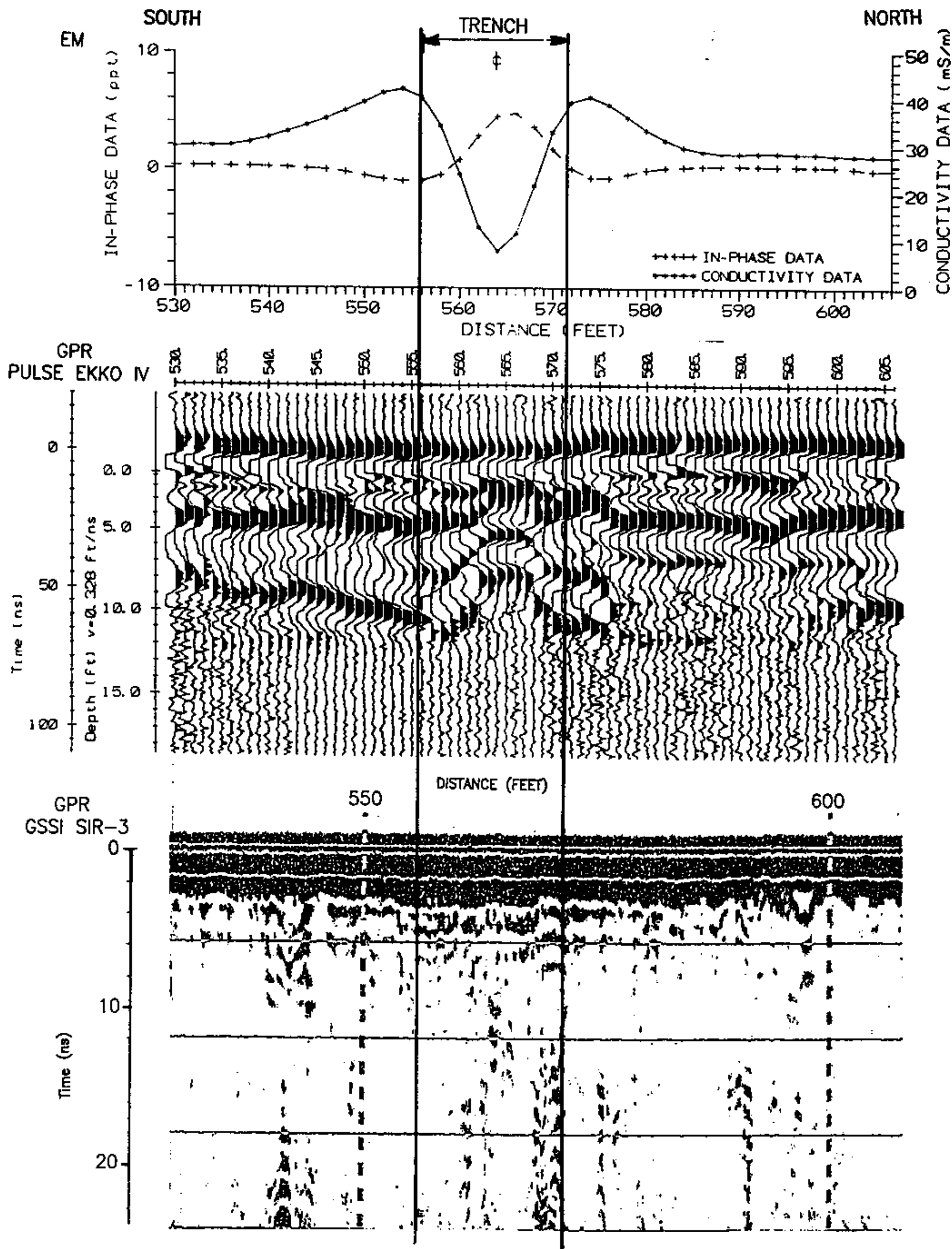
FIGURE 3.6 COMPARISON OF EM AND GPR PROFILES SWMU B-2
