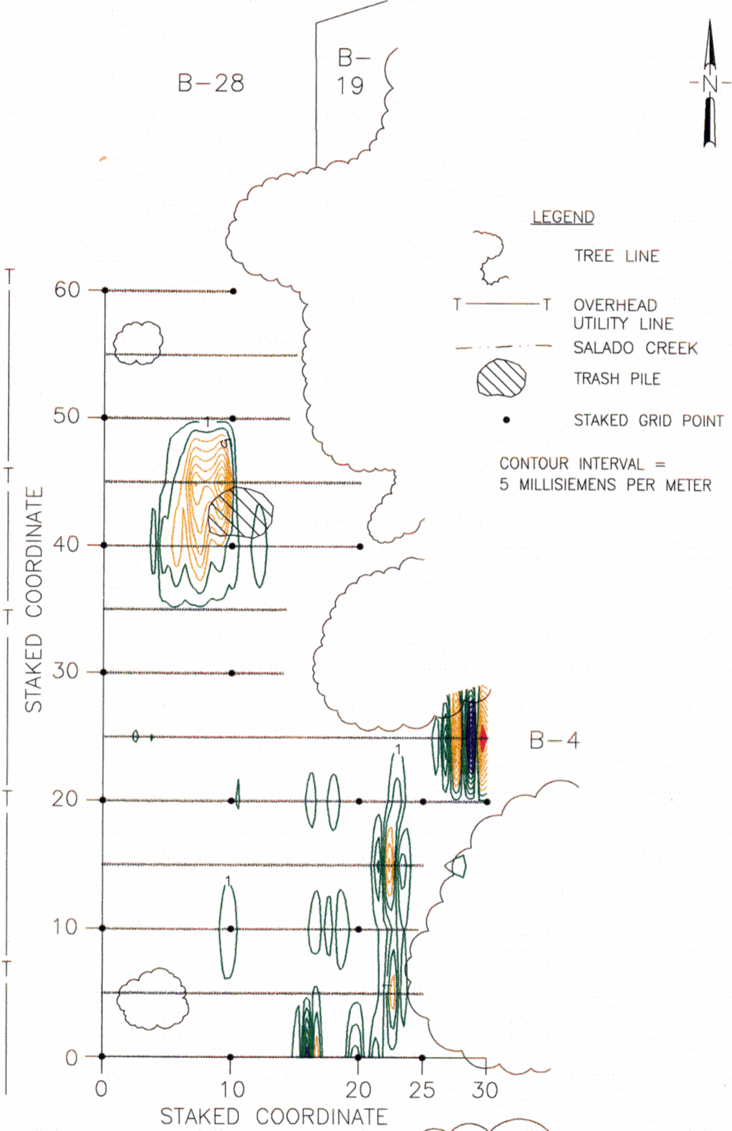
FIGURE 11.35 EM IN-PHASE DATA (E-W) SALADO CREEK CSSA GROUNDWATER EVALUATION
