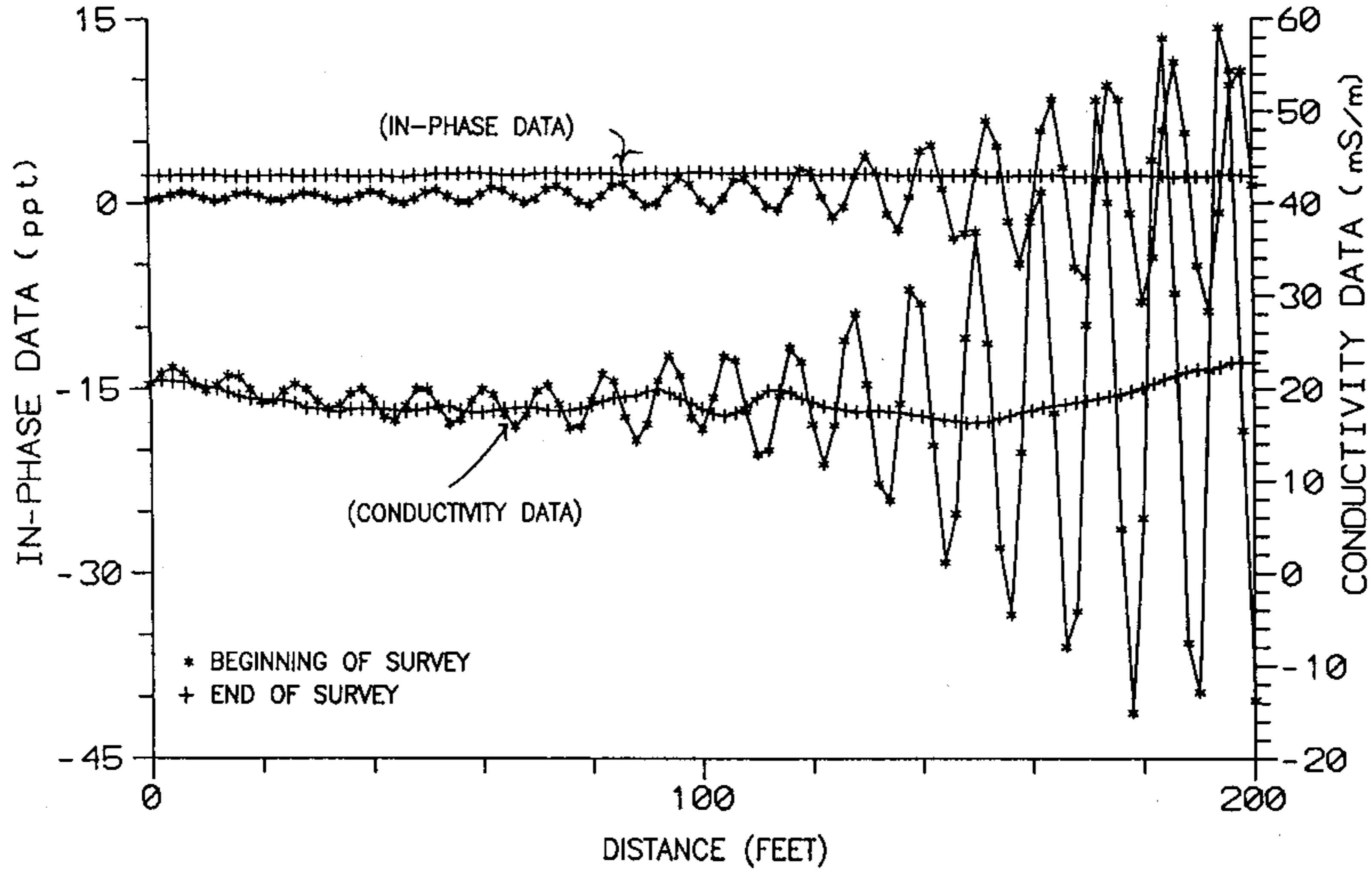
FIGURE 11.12 SOUTH PASTURE EM QC LINE (E-W) CSSA GROUNDWATER EVALUATION
