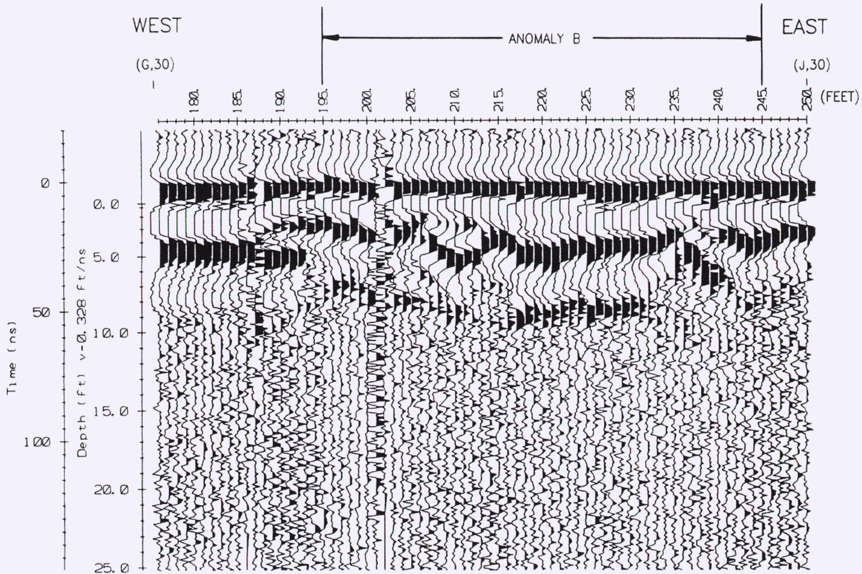
FIGURE 9.5 PULSE EKKO IV GPR PROFILE SWMU B-24 CSSA HIGH PRIORITY SWMUs
