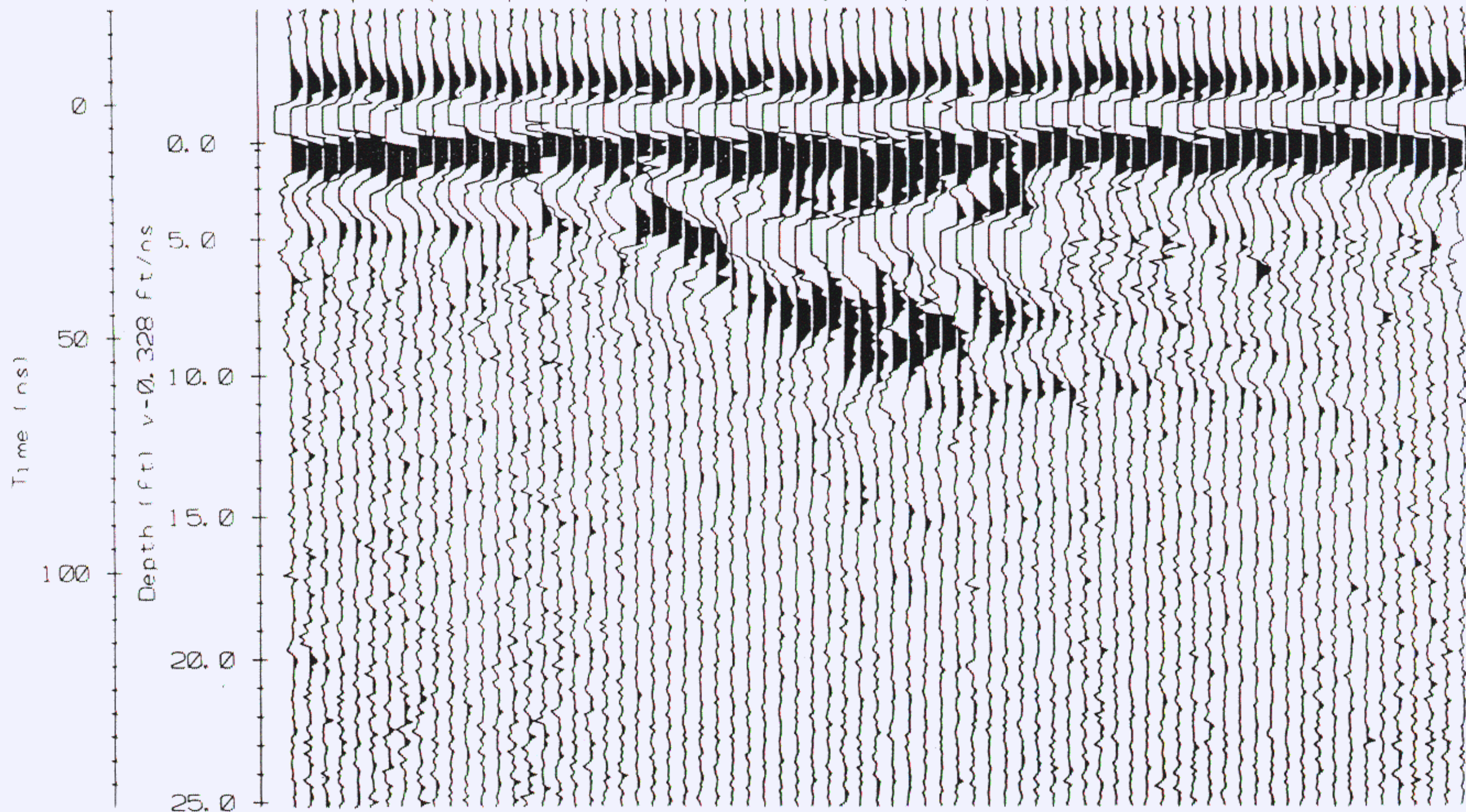
FIGURE 6.5 PULSE EKKO IV GPR PROFILE SWMU B-15/16 CSSA HIGH PRIORITY SWMUs
