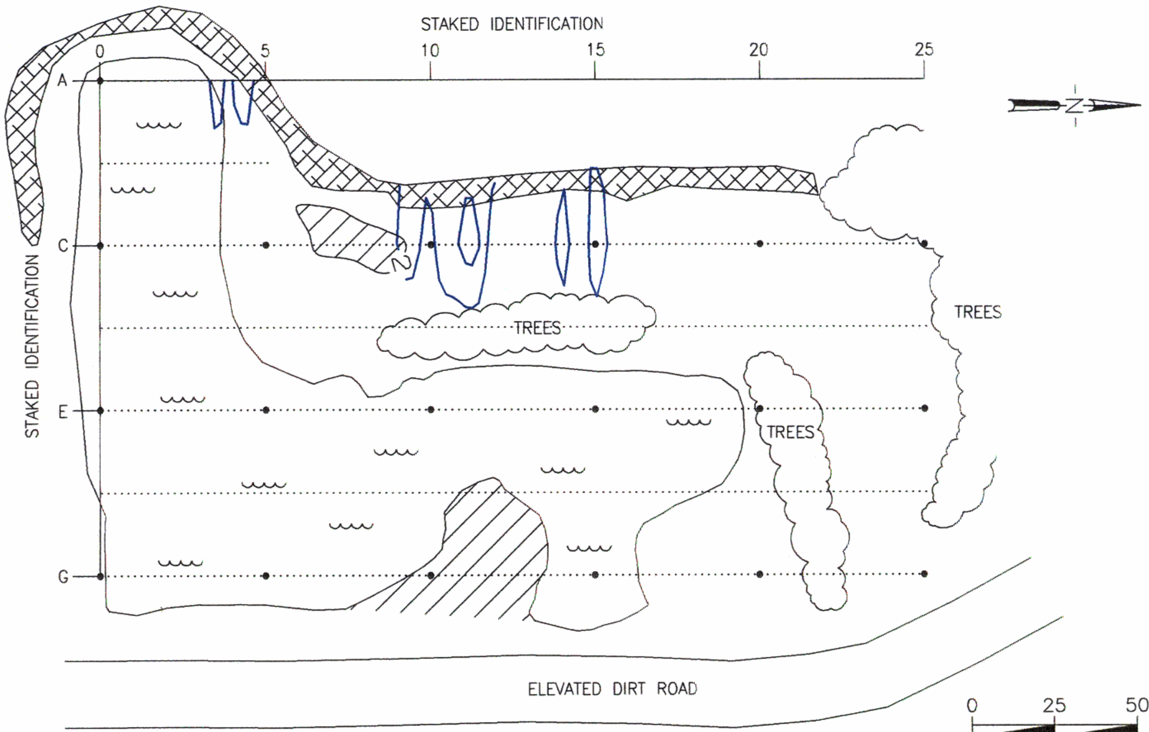
FIGURE 5.3 EM IN-PHASE DATA (N-S) SWMU B-12 CSSA HIGH PRIORITY SWMUs
