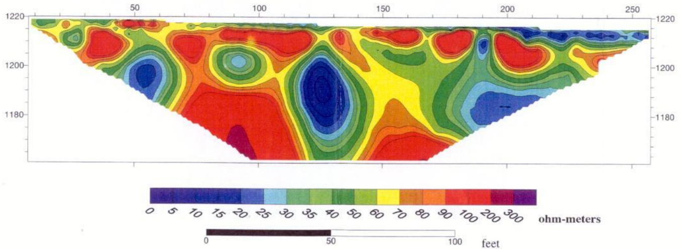
Model resistivity section - 7.7% Inversion RMS error
