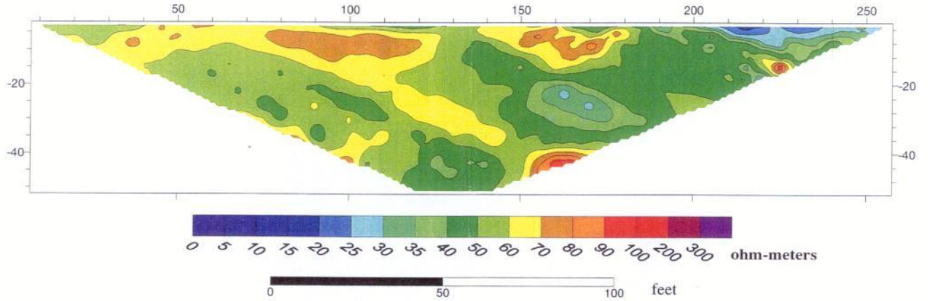
Measured apparent resistivity section
