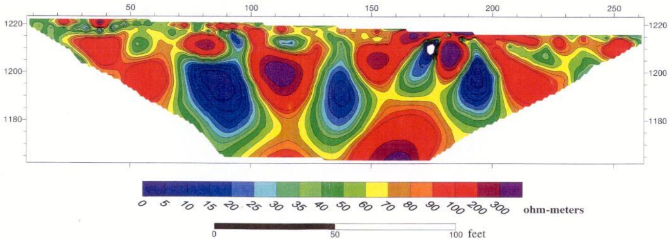
Model resistivity section - 8.1% Inversion RMS error
