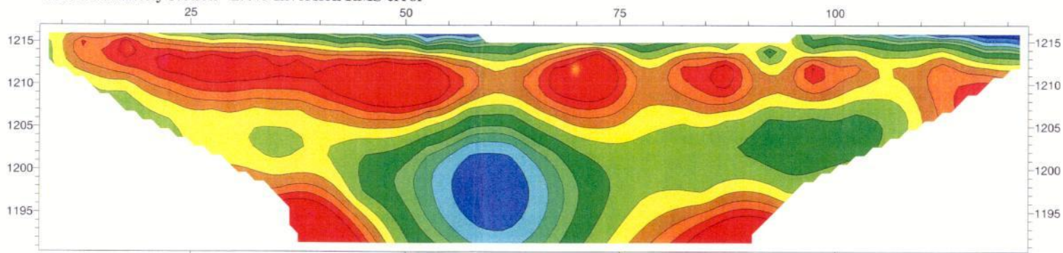
Model resistivity section - 2.4% Inversion RMS error
