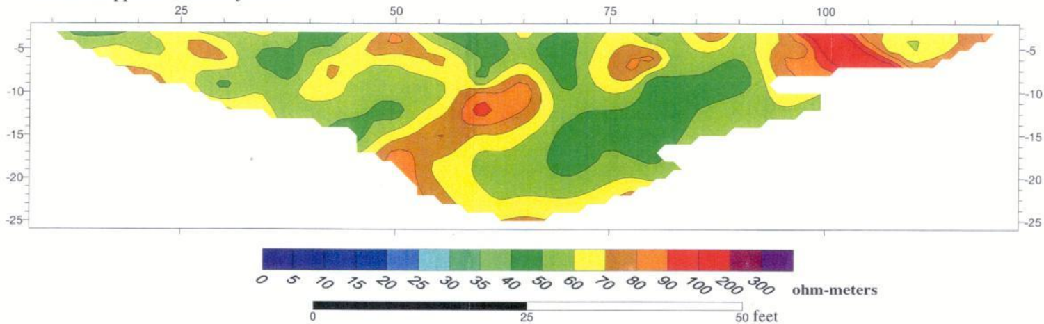
Measured apparent resistivity section
