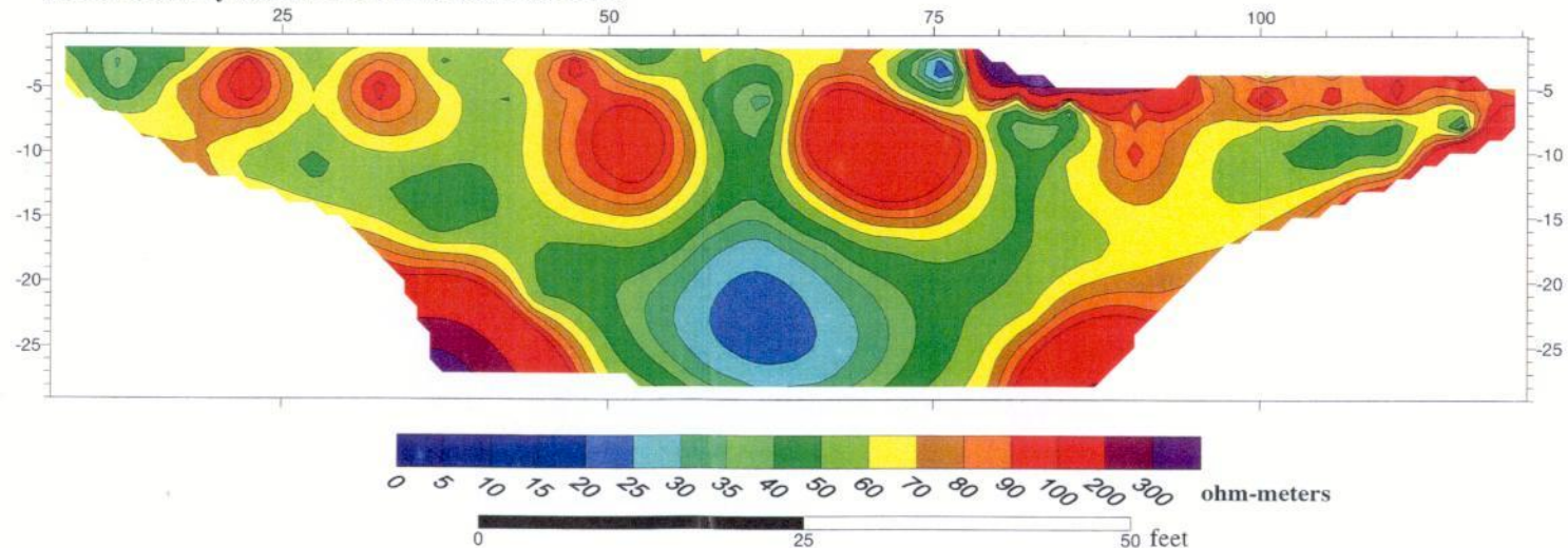
Model resistivity section - 4.8% Inversion RMS error
