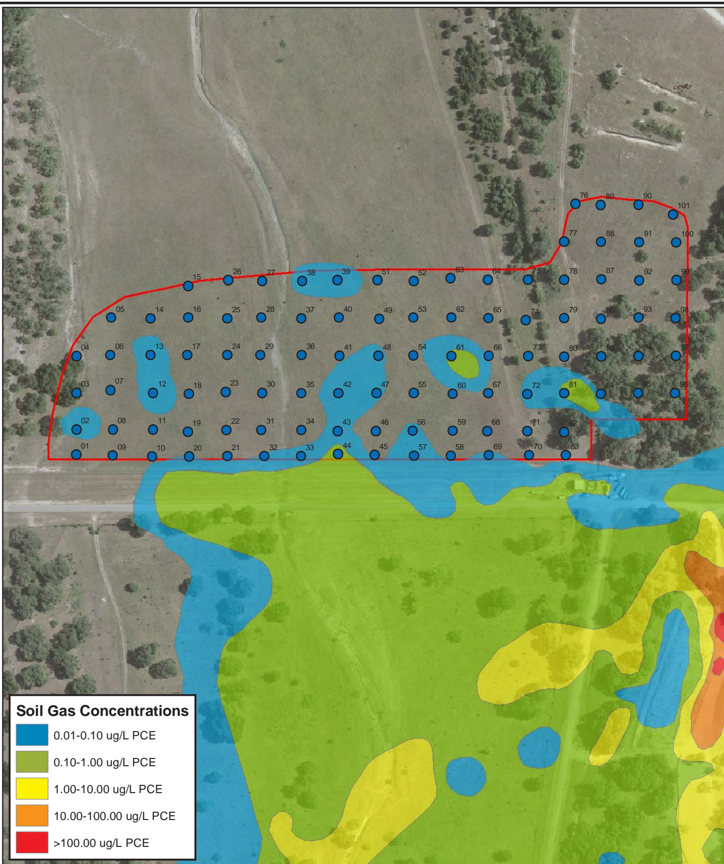
Figure AOC66-7 Soil Gas Plume Map Camp Stanley Storage Activity PARSONS
