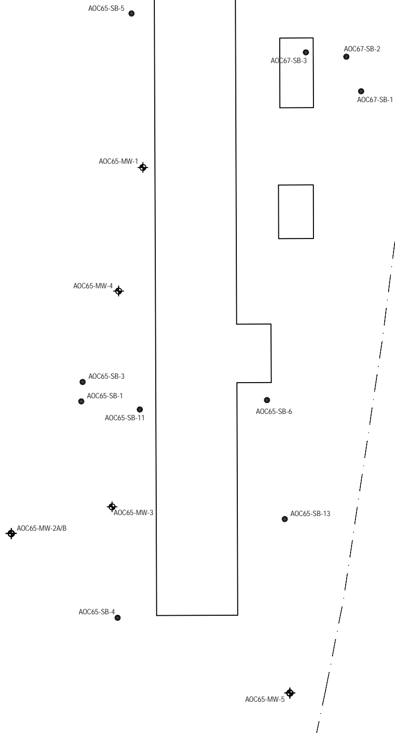
Figure 4.1 AOC 65 Soil Gas Survey Soil Borings and Well Locations Camp Stanley Storage Activity PARSONS ENGINEERING SCIENCE, INC.
