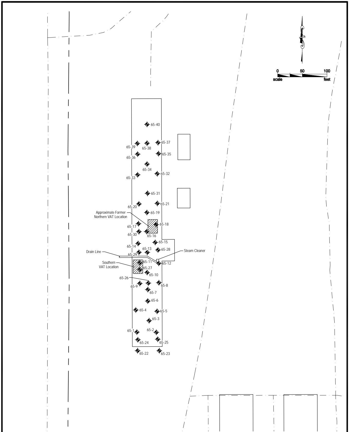
Figure 2.4 AOC 65, Inside Building 90, Soil Gas Survey Sample Location Map Camp Stanley Storage Activity PARSONS ENGINEERING SCIENCE, INC.
