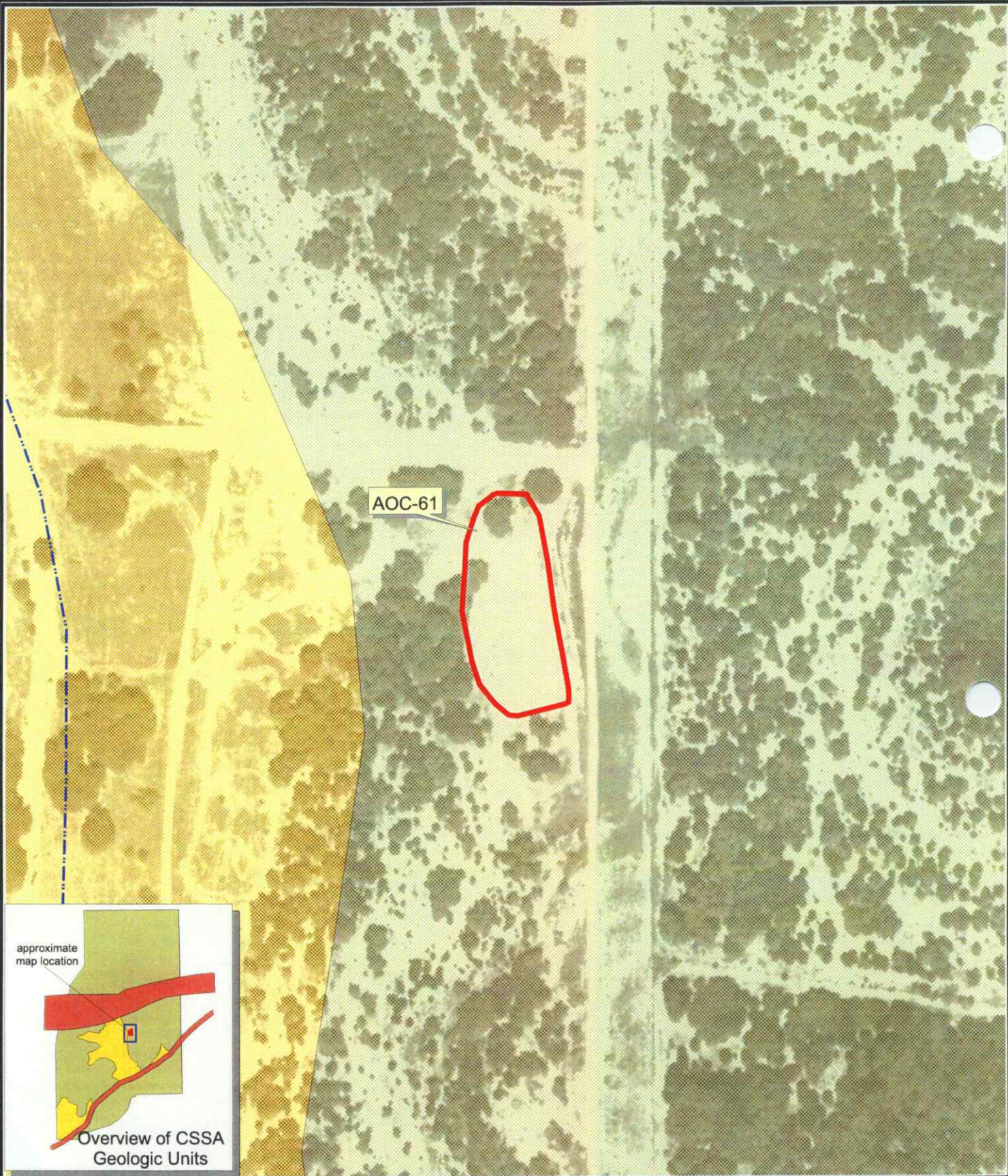
Figure AOC61-5 Geologic Setting Camp Stanley Storage Activity PARSONS
