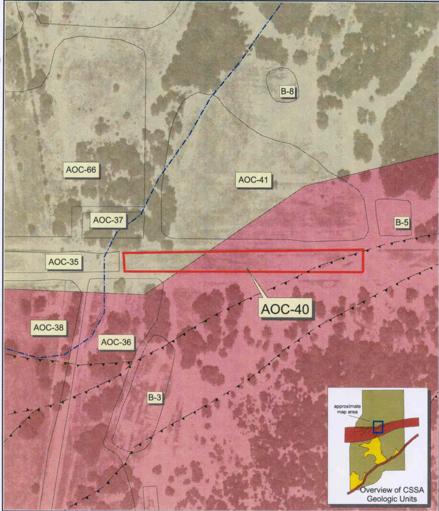
Figure AOC40-3 Geologic Setting Camp Stanley Storage Activity PARSONS ENGINEERING SCIENCE, INC.
