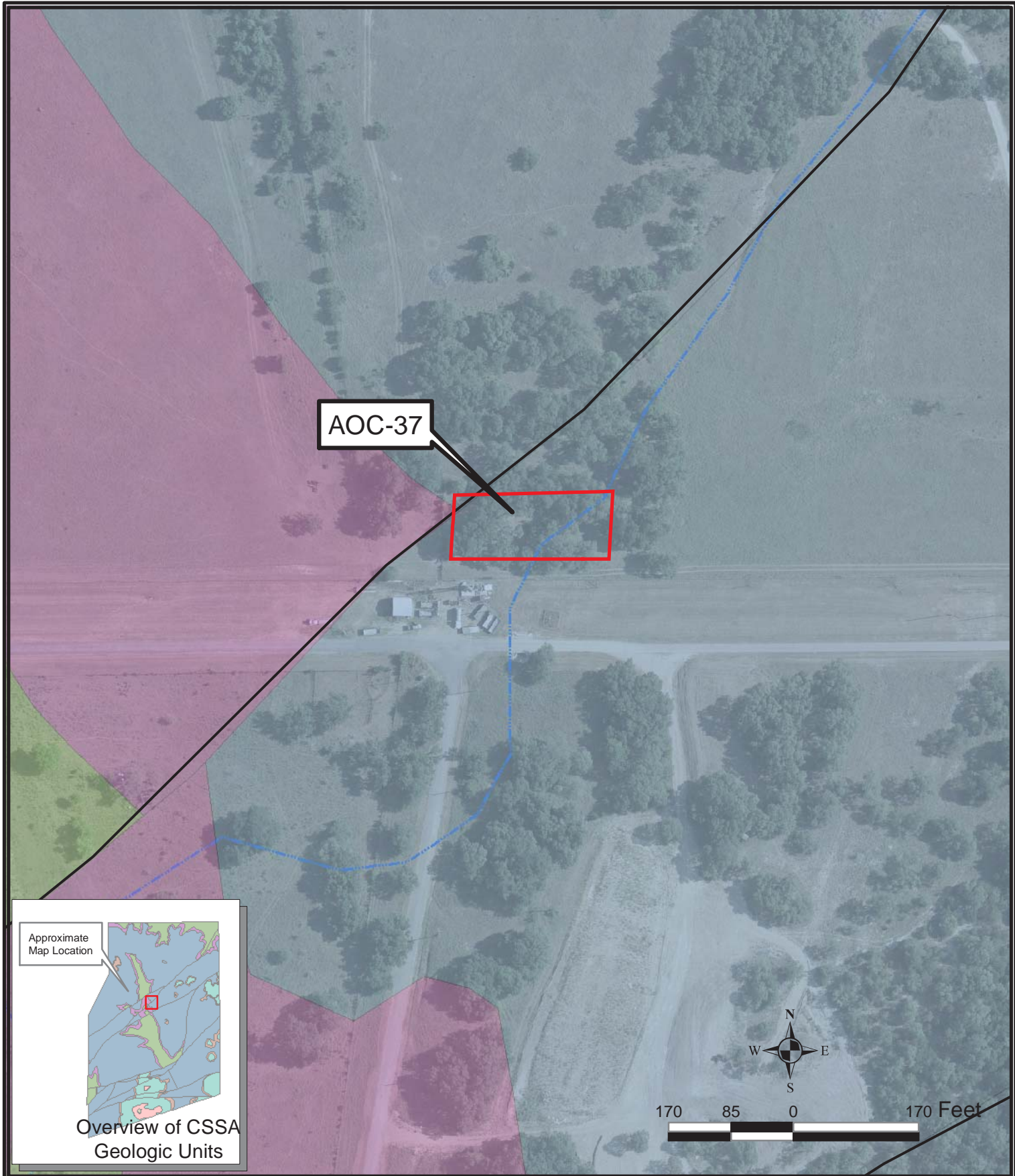
Figure: AOC37-6 Geologic Setting Camp Stanley Storage Activity PARSONS
