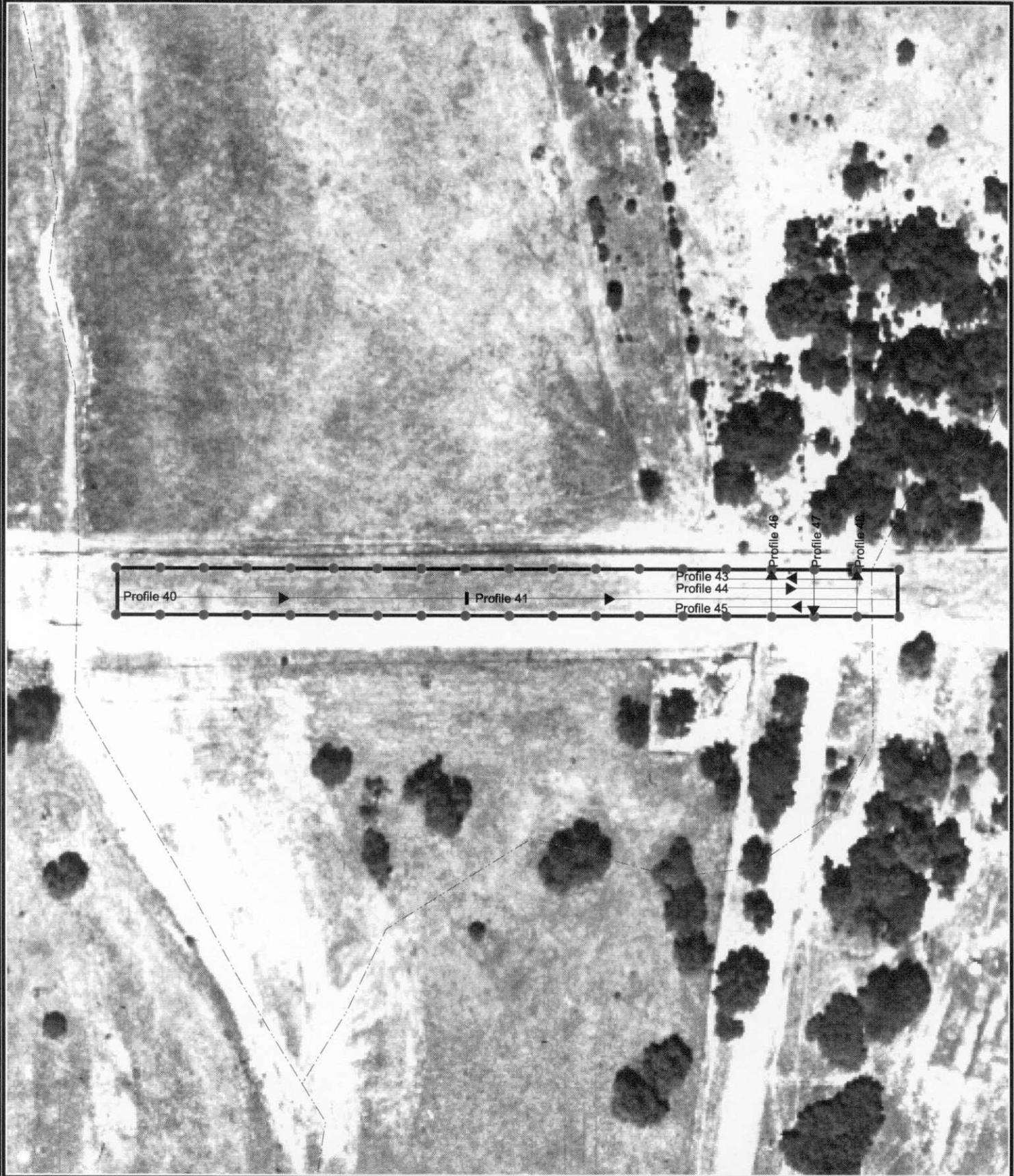
Figure AOC35-6 Geophysical Survey Grid And GPR Profile Locations Camp Stanley Storage Activity PARSONS ENGINEERING SCIENCE, INC.
