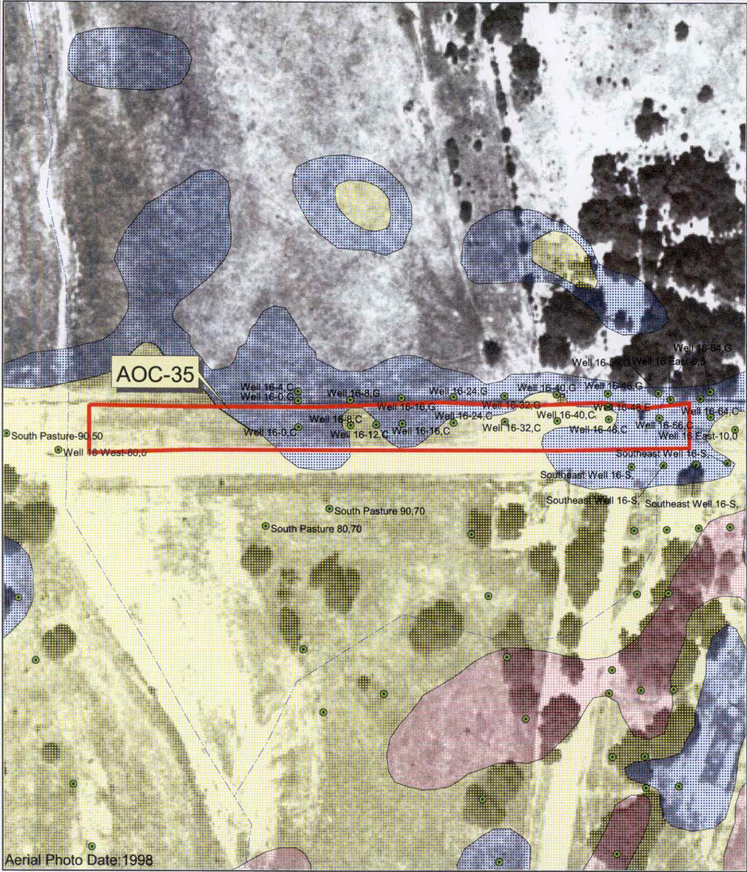
Figure AOC35-5 PCE Soil Gas Contour Map Camp Stanley Storage Activity PARSONS ENGINEERING SCIENCE, INC.
