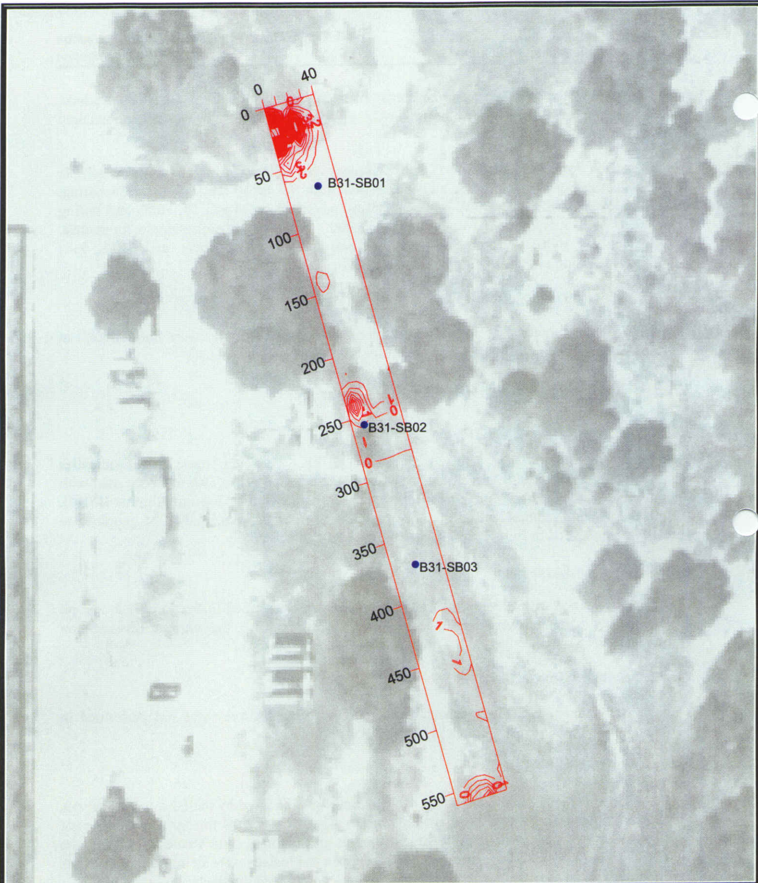
Figure B31-7 Electromagnetic Data In-Phase Camp Stanley Storage Activity PARSONS ENGINEERING SCIENCE, INC.
