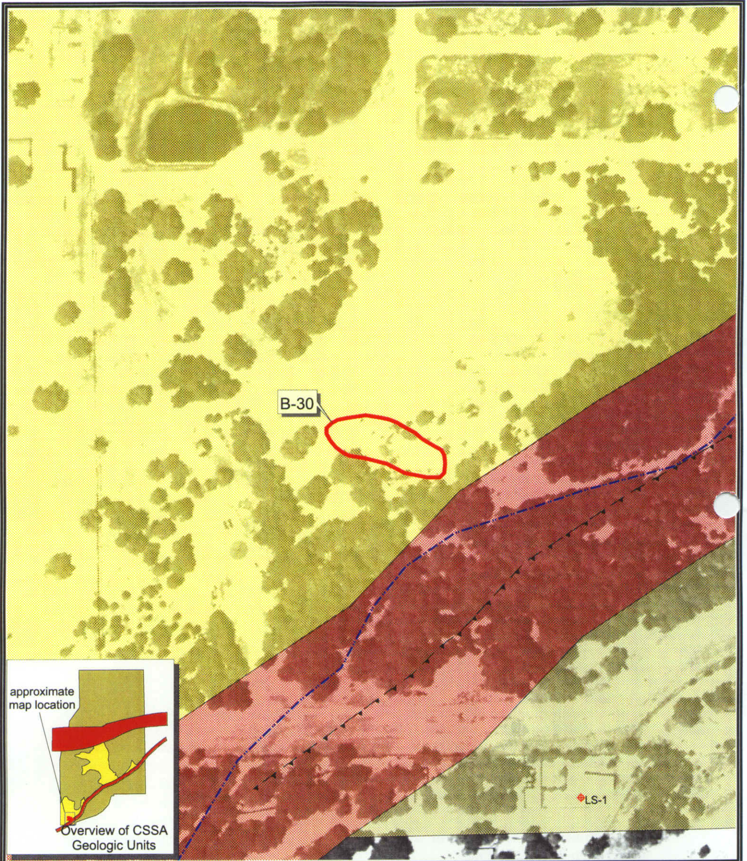
Figure B30-3 Geologic Setting Camp Stanley Storage Activity PARSONS ENGINEERING SCIENCE, INC.
