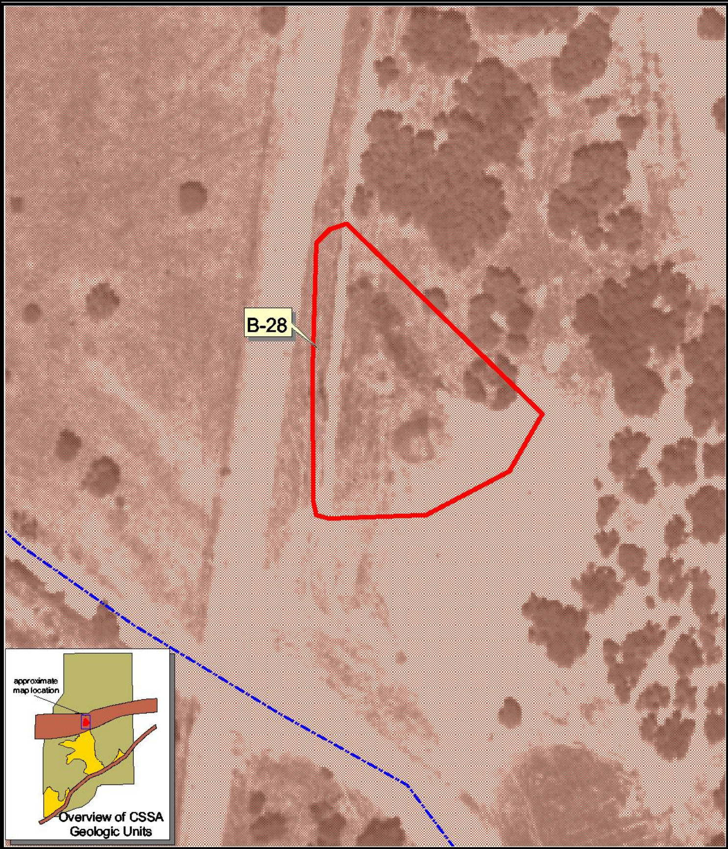
Figure B28-3 Geologic Setting Camp Stanley Storage Activity PARSONS ENGINEERING SCIENCE, INC.
