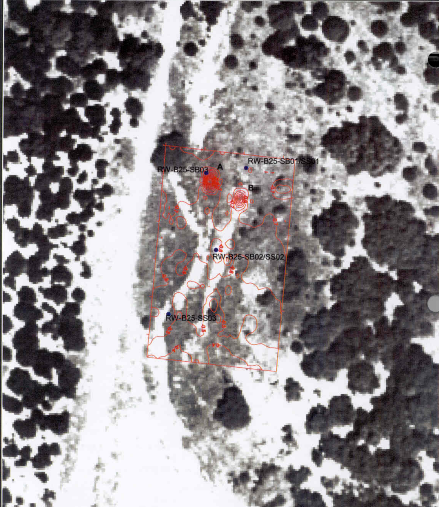
Figure B25-5 Electromagnetic Data In-Phase Camp Stanley Storage Activity PARSONS ENGINEERING SCIENCE, INC.
