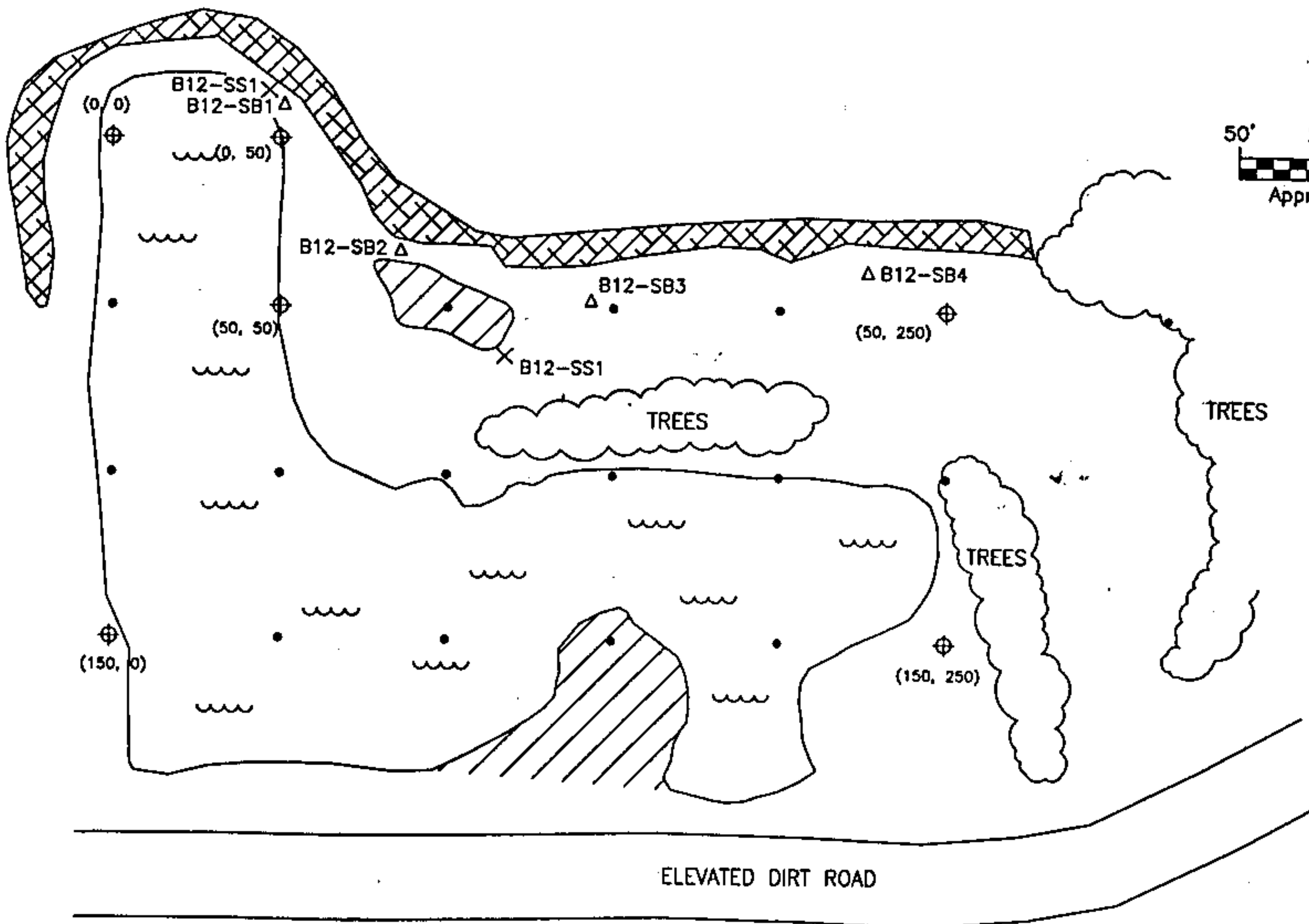
FIGURE B12-1 SWMU B-12 SITE MAP CAMP STANLEY STORAGE ACTIVITY PARSONS ENGINEERING SCIENCE, INC.
