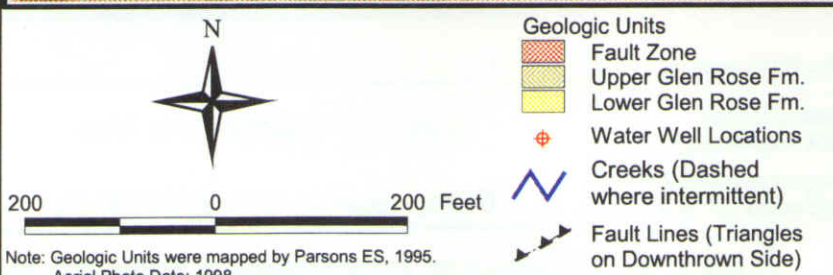
Figure B11-3 Geologic Setting Camp Stanley Storage Activity PARSONS ENGINEERING SCIENCE, INC.
