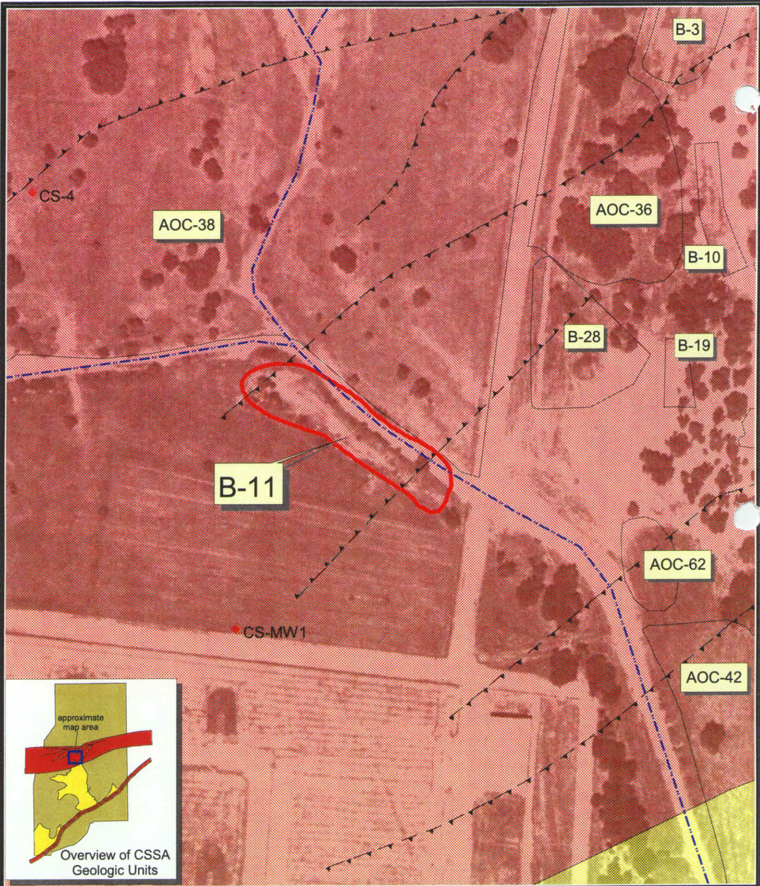
Figure B11-3 Geologic Setting Camp Stanley Storage Activity PARSONS ENGINEERING SCIENCE, INC.
