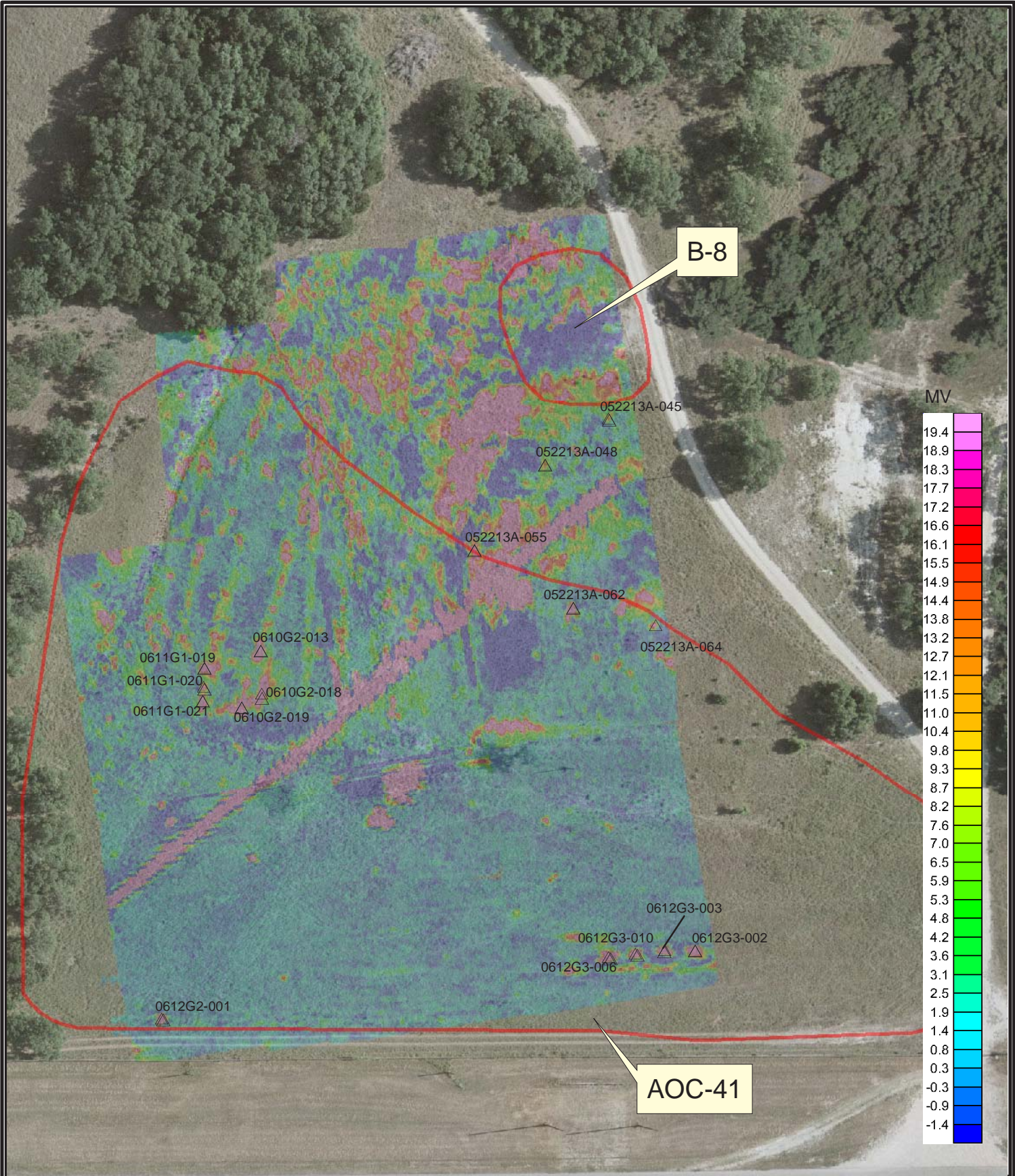
Figure B8-7 B8 Geophysical Survey Geonics EM-61 MK2 Ch. 3 Gridded Data
