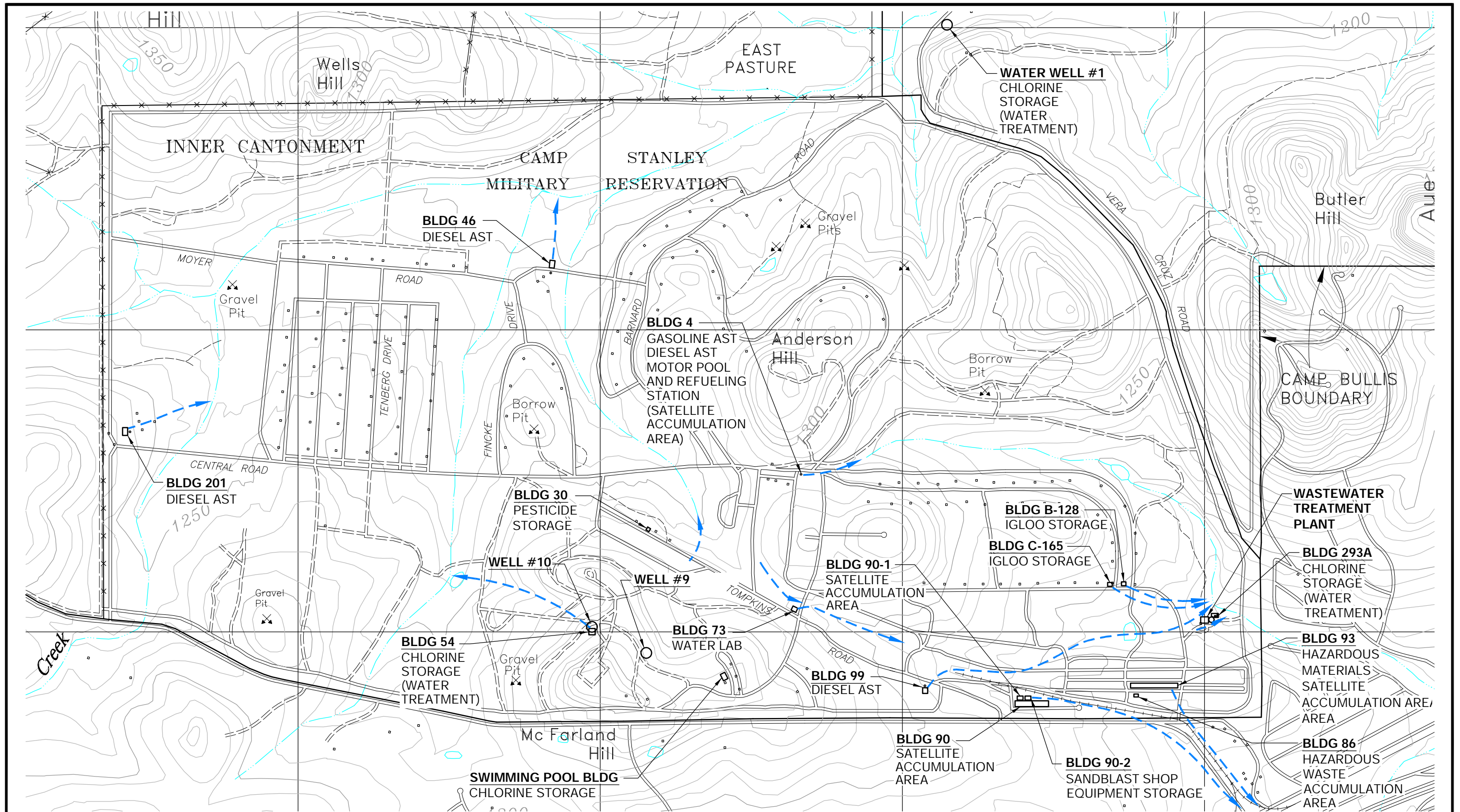
Figure 2.1 Site Drainage June 2001 Camp Stanley Storage Activity PARSONS ENGINEERING SCIENCE, INC.
