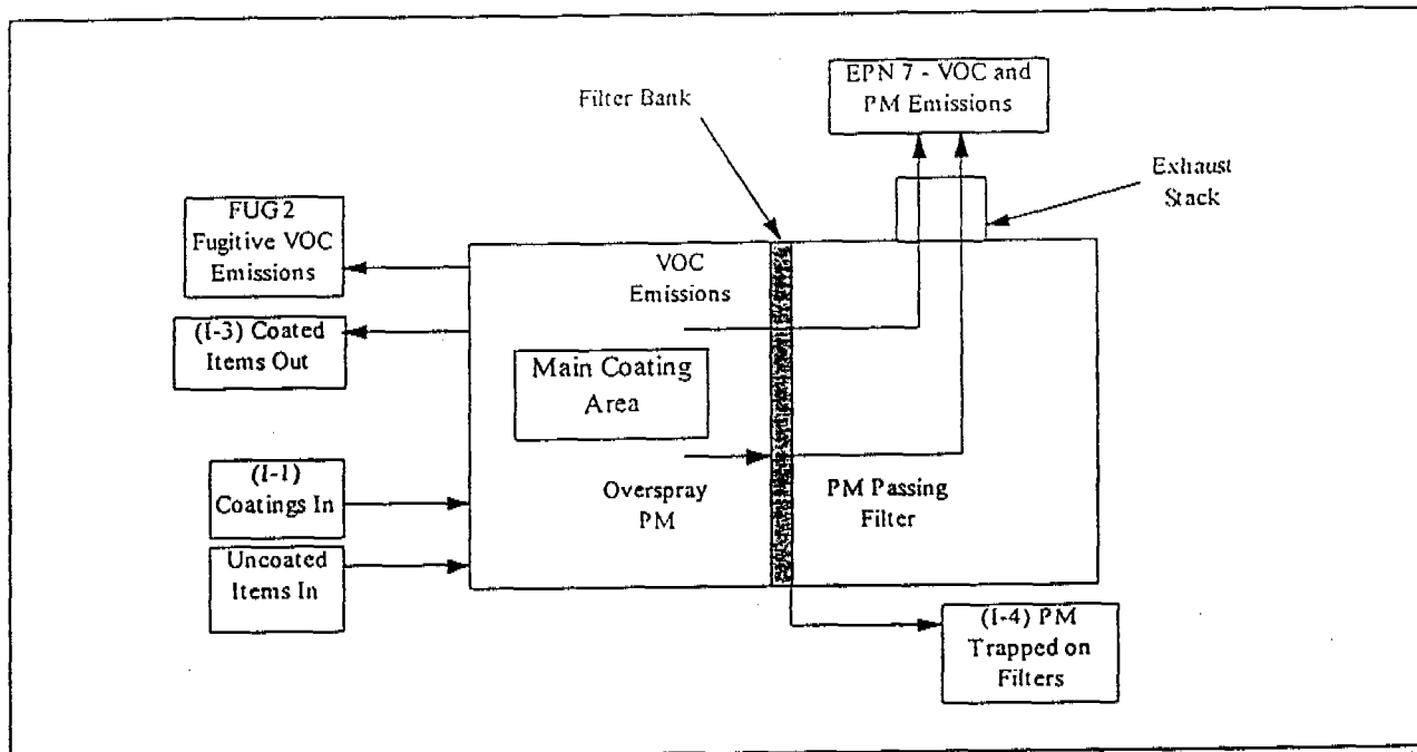
Figure IV.1. Process Flow Diagram for Paint Booth - Building 27
