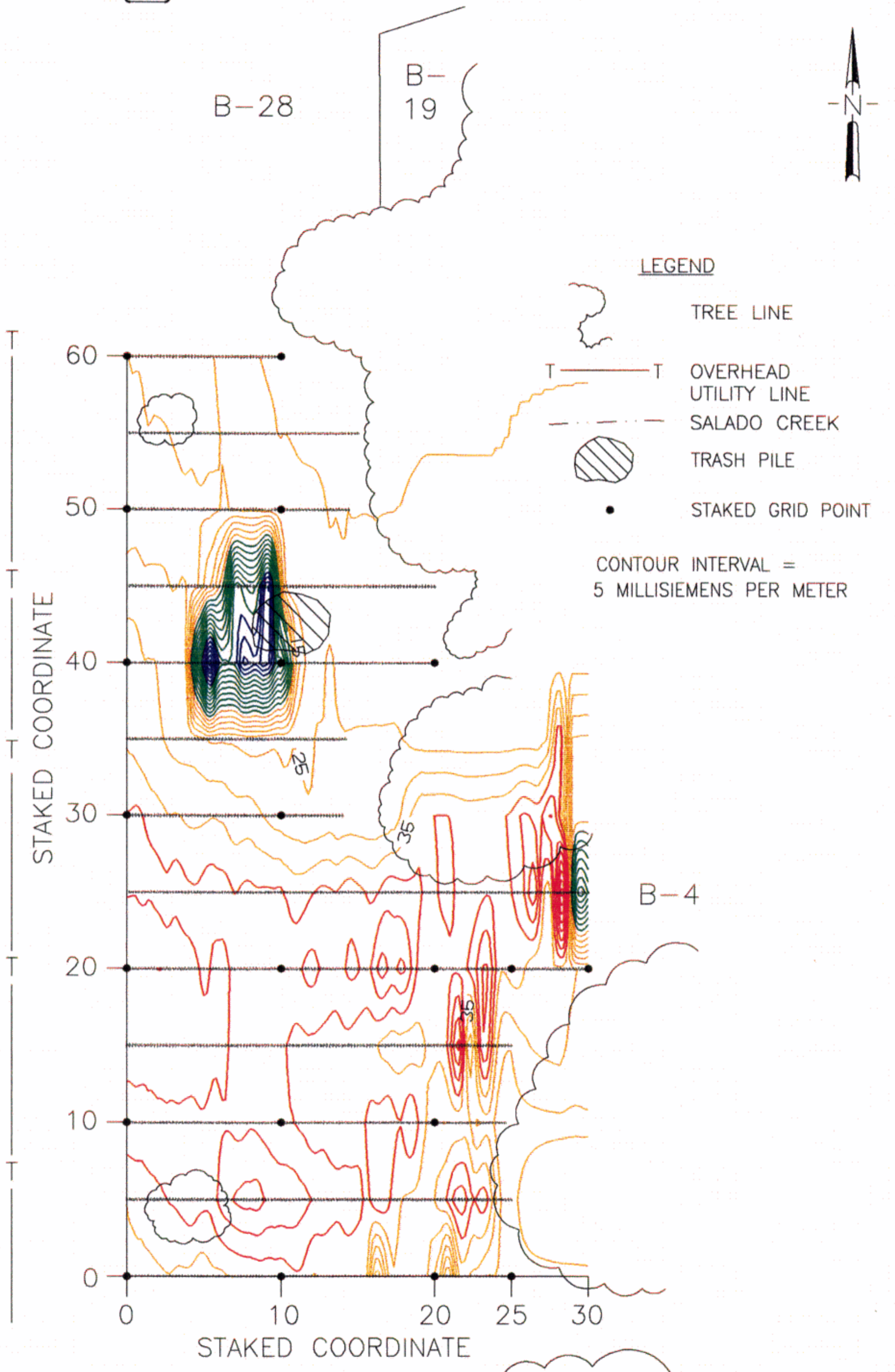
FIGURE 11.34 EM CONDUCTIVITY DATA (E-W) SALADO CREEK CSSA GROUNDWATER EVALUATION
