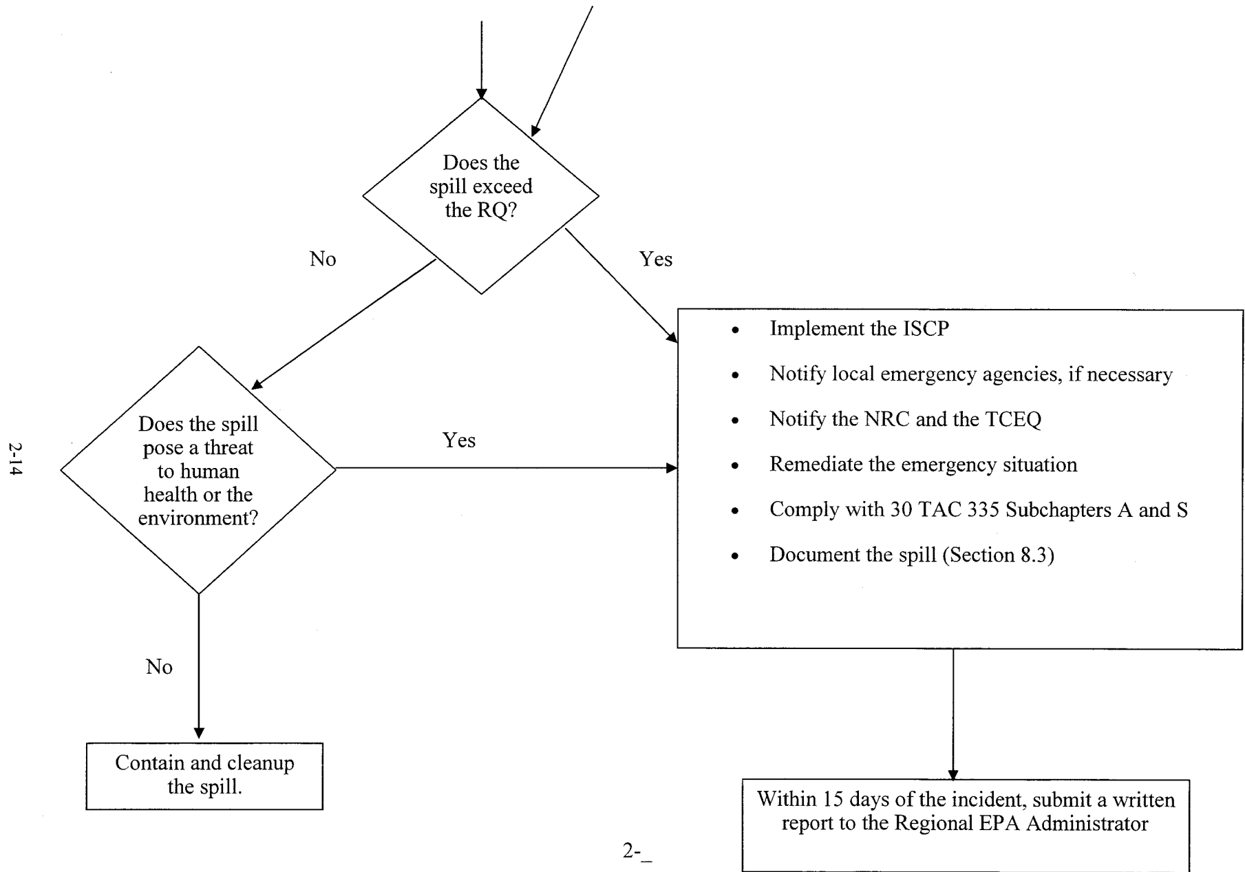
Figure 2.2 Flow Diagram for Response to Emergency Situations
