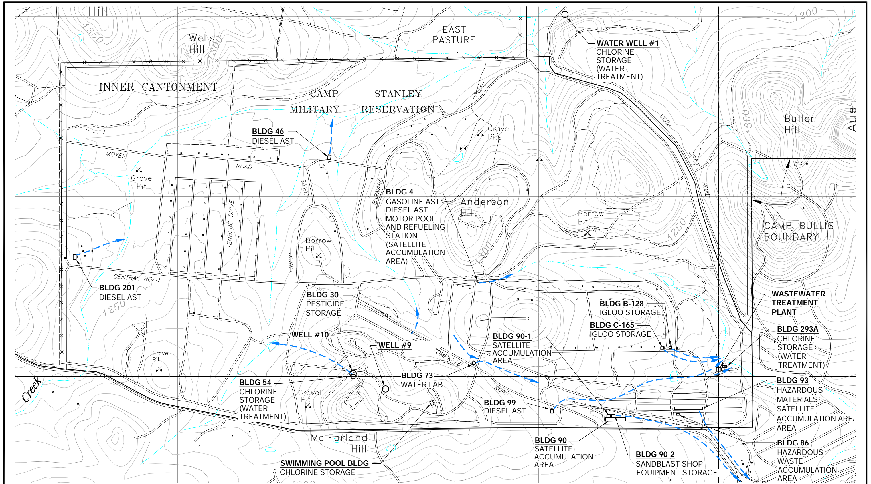
Figure 4.1 Sites Where Releases May Occur June 2001 Camp Stanley Storage Activity PARSONS ENGINEERING SCIENCE, INC.
