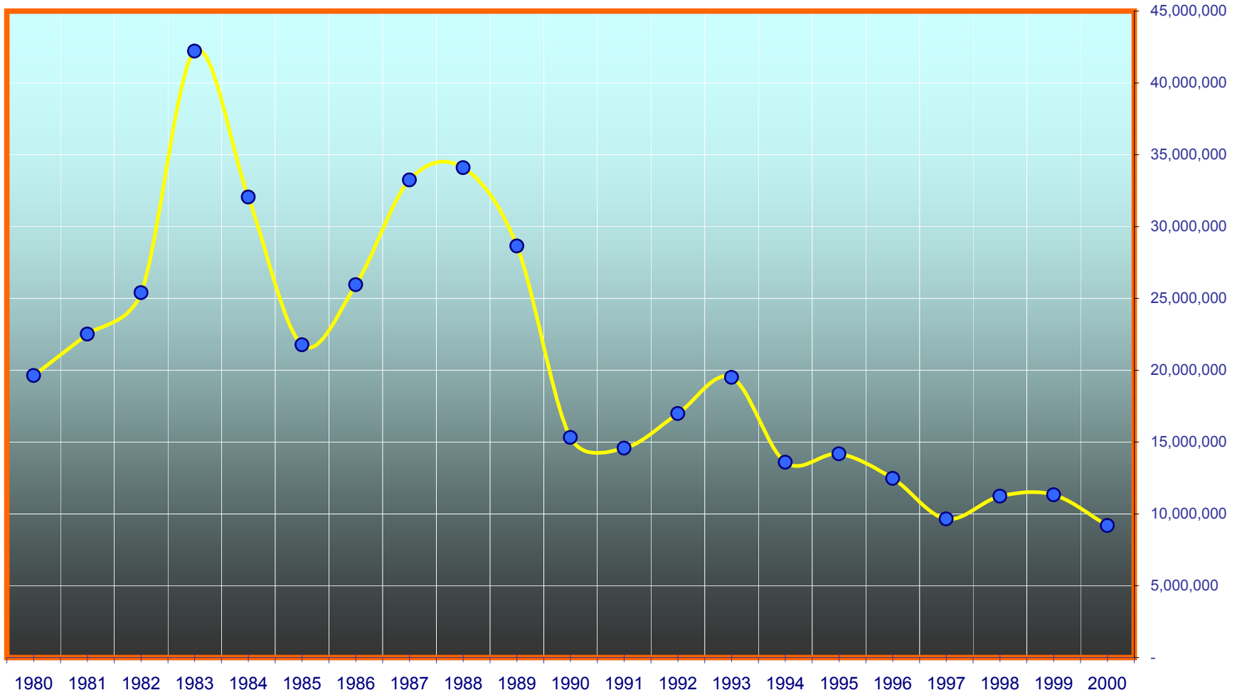
Figure 3 Annual Pumping 1980-2000 (in gallons)
