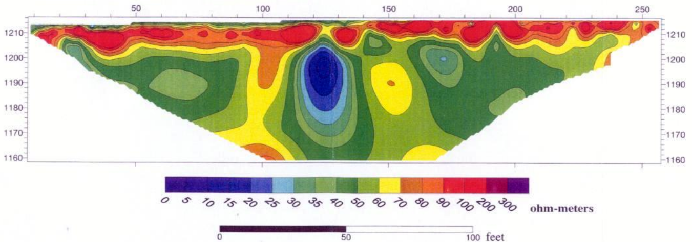
Model resistivity section - 3.7% Inversion RMS error
