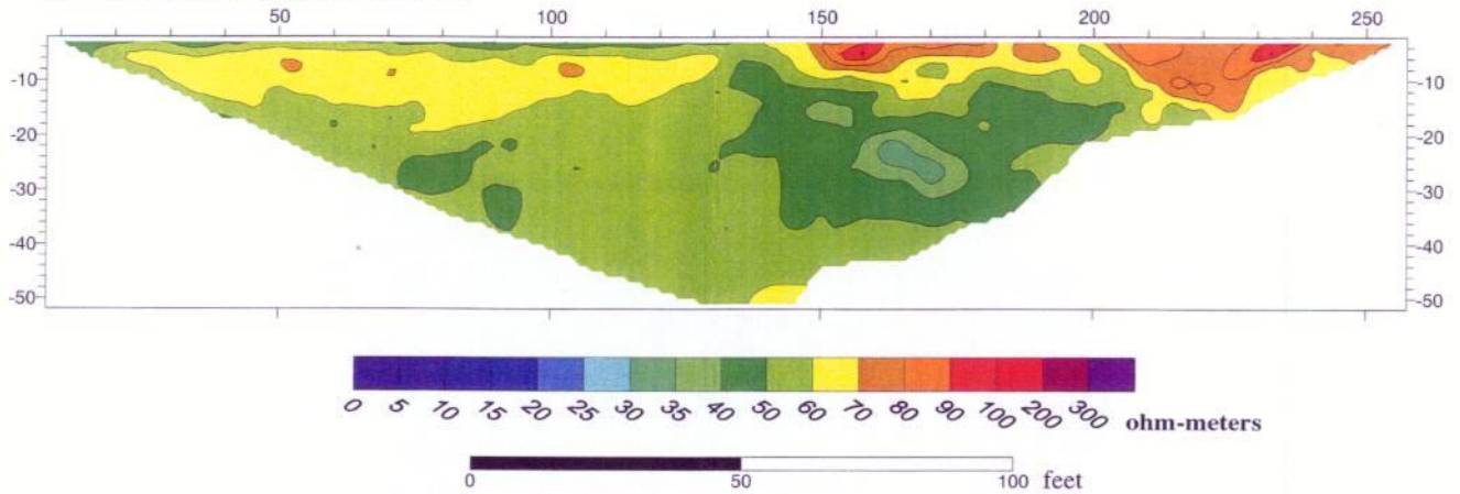
Measured apparent resistivity section
